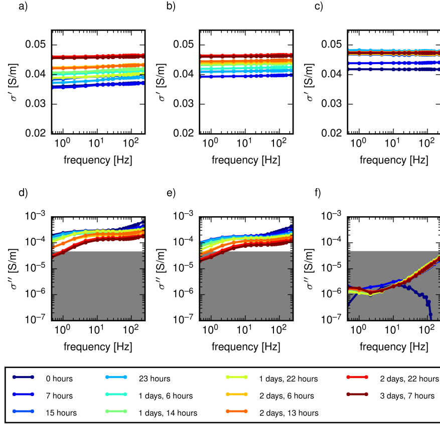
Figure 7. Intrinsic complex conductivity spectra (in terms of real component \sigma' and imaginary component \sigma'' ) for all time steps (indicated by colour color of the curves) recovered from the multi-frequency inversion results at different locations in the rhizotron: a,d) stem area ( x position: 20.25 cm, z position: -0.75 cm ); b,e) bottom of the root system ( x position: 20.25 cm, z position -6.25 cm ); c,f) water-only location ( x position: 20.25 cm, z position: -50.25 cm ). Positions for a/d and b/e are also indicated in Fig. 4a. Values of \sigma'' that lie below the measurement accuracy of the system (1 mrad phase shift at 1 kHz for water, see Zimmermann et al. (2008) ) are indicated by gray areas.
