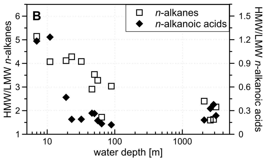
Figure S1: The ratios of high- over low-molecular weight n -alkanes and n -alkanoic acids decrease along the transect due to dilution with marine OC.
