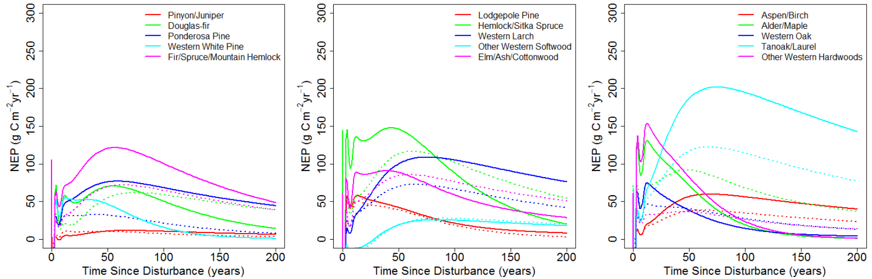
Fig. S2 Post-fire characteristic trajectories of NEP in the PNW region. Solid lines are plotted for high site productivity, and dashed lines for low productivity. Figures in the first row are plotted for low severity fire, second row for medium severity fire, and the third row for high severity fire.
