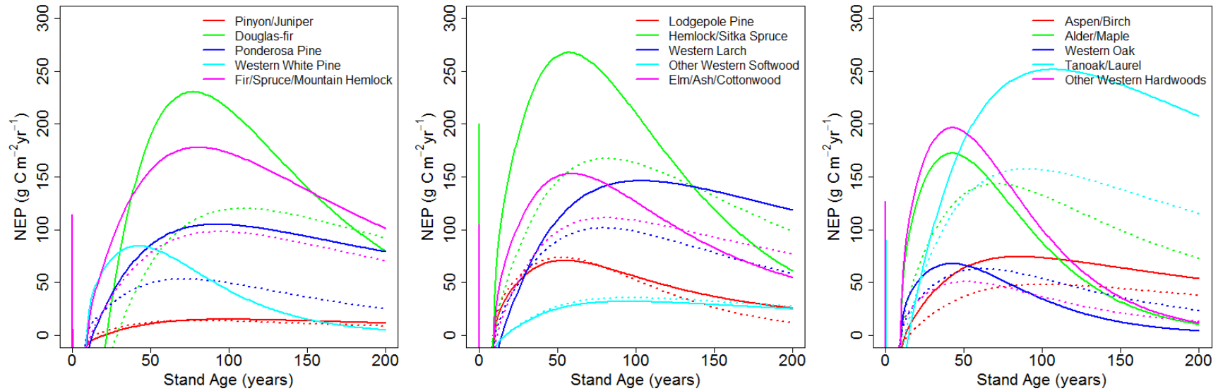
Fig. S1 Characteristic NEP trajectories following a stand-replacing disturbance in the PNW region. Solid lines are plotted for high site productivity, and dashed lines for low productivity.
