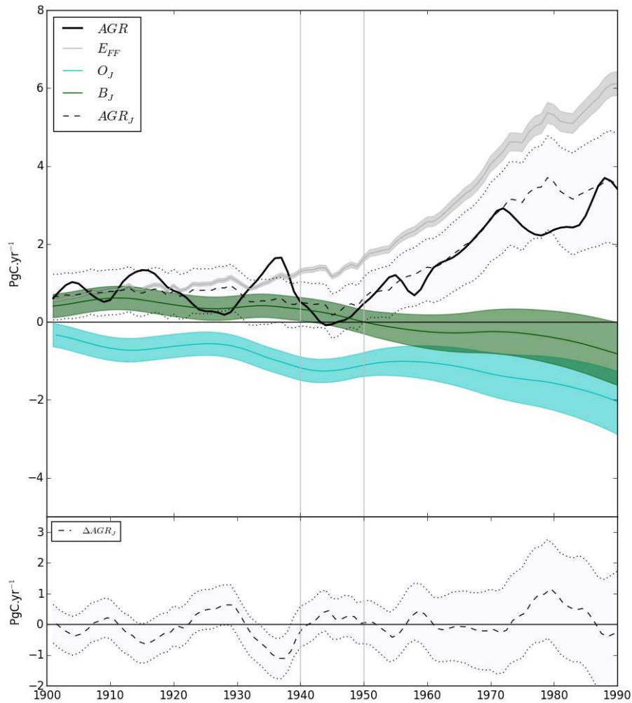
Figure 2. Atmospheric CO 2 growth rate ( AGR ) from the observational record, calculated from the spline fit in Figure 1 (black line, top panel). Fossil fuel emissions from the CDIAC database and respective uncertainty ( E_{FF} ), and the reconstruction of ocean and biospheric fluxes from Joos et al. (1999), O_J and B_J respectively (filled areas in top panel). The resulting balance from the latter three datasets ( AGR_J ) and uncertainty is shown in the top panel (dashed and dotted lines, respectively), and the corresponding difference between AGR and AGR_J is shown in the bottom panel.
