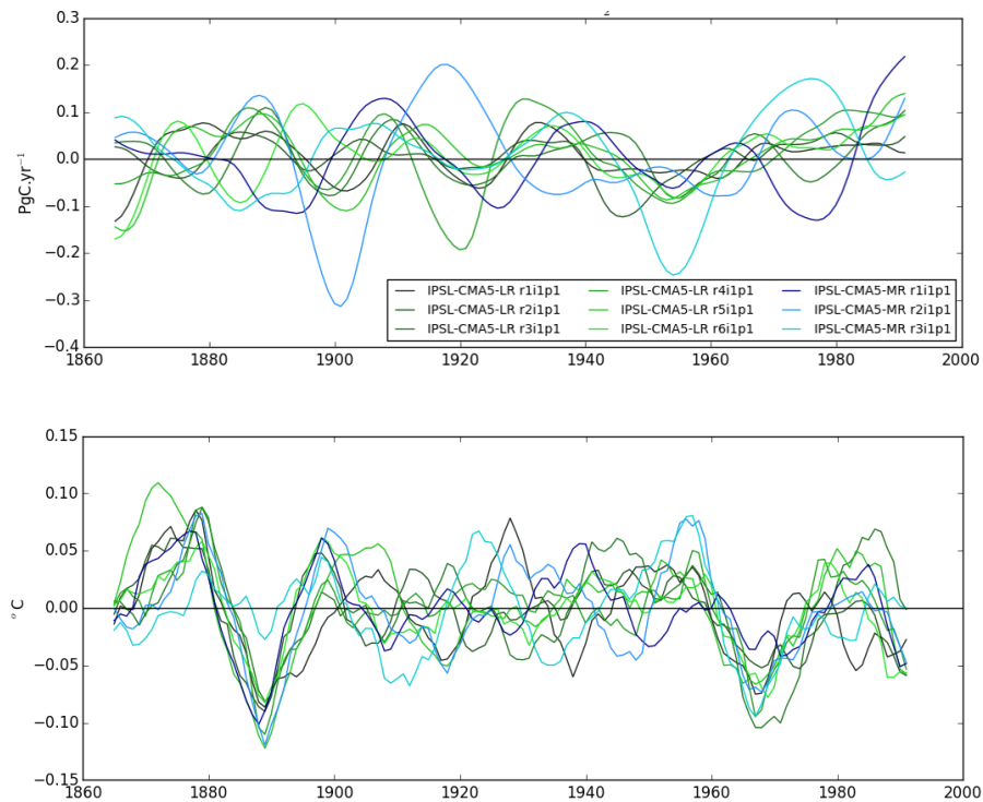
Figure 5. As in Figure 4, but for six different realisations from IPSL-CM5A-LR and three from IPSL-CM5A-MR (top panel) and the corresponding SST temperature anomalies in the Nino3.4 region. The SST anomaly is calculated as the 10-yr moving average departure of the SST data from a 30-yr long reference period.
