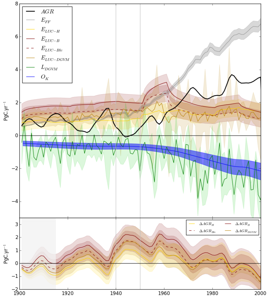
Figure 3. As in Figure 2 but for the independent estimates of sources and sinks: E_{FF} from CDIAC, E_{LUC} from Houghton (H), BLUE (B) and BLUE with lower C-stock changes (Blc) and DGVMs forced with LUC, ocean from Khatiwala et al. (2009) reconstruction and land-sink as estimated by DGVMs forced only by CO 2 and climate. In the bottom panel, the difference between observed AGR and AGR_H , AGR_B , AGR_{Blc} and AGR_{DGVM} is shown.
