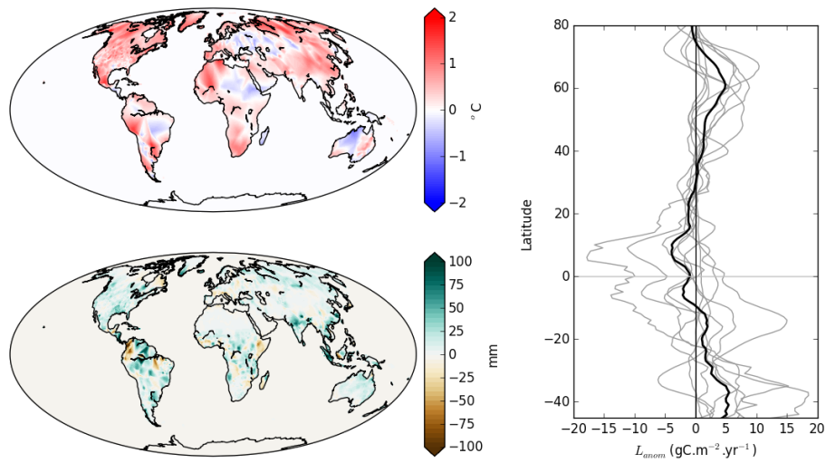
Figure 6. Response of the terrestrial ecosystems to the climate anomalies during the plateau period, simulated by the DGVMs. Temperature (left top) and precipitation (left bottom) anomaly fields during 1940-50 (relative to 1900-1930), and the corresponding latitudinal anomaly of L_{DGVM} estimated by each model (grey lines) and the multi-model average (right panel).
