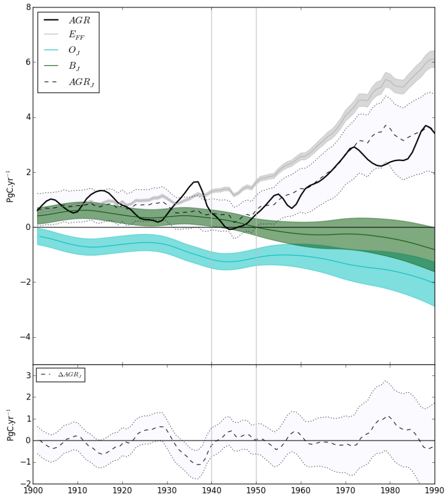
Figure 2. Atmospheric \text{CO}_2 growth rate ( AGR ) from the observational record, calculated from the spline fit in Figure 1 (black line, top panel). Fossil fuel emissions from the CDIAC database and respective uncertainty ( E_{FF} ), and the reconstruction of ocean and biospheric fluxes from Joos et al. (1999), O_J and B_J respectively (filled areas in top panel). The resulting balance from the latter three datasets ( AGR_J ) and uncertainty is shown in the top panel (dashed and dotted lines, respectively), and the corresponding difference between AGR and AGR_J is shown in the bottom panel.
