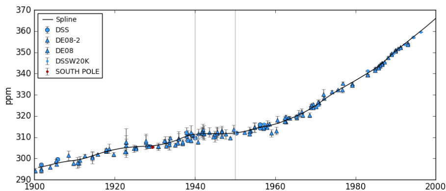
Figure 1. Atmospheric CO_2 concentration in the Law Dome ice core and firn record from Rubino et al. (2013) and respective uncertainties (markers and whiskers), and the spline-fit applied to the data following Enting et al. (2006), which attenuates by 50% variations of c.a. 23 years. The period corresponding to the plateau is highlighted between vertical grey lines. The blue markers correspond to samples from Law Dome and red markers from South Pole; different symbols indicate the different ice-cores (big markers) and firn samples (dots).
