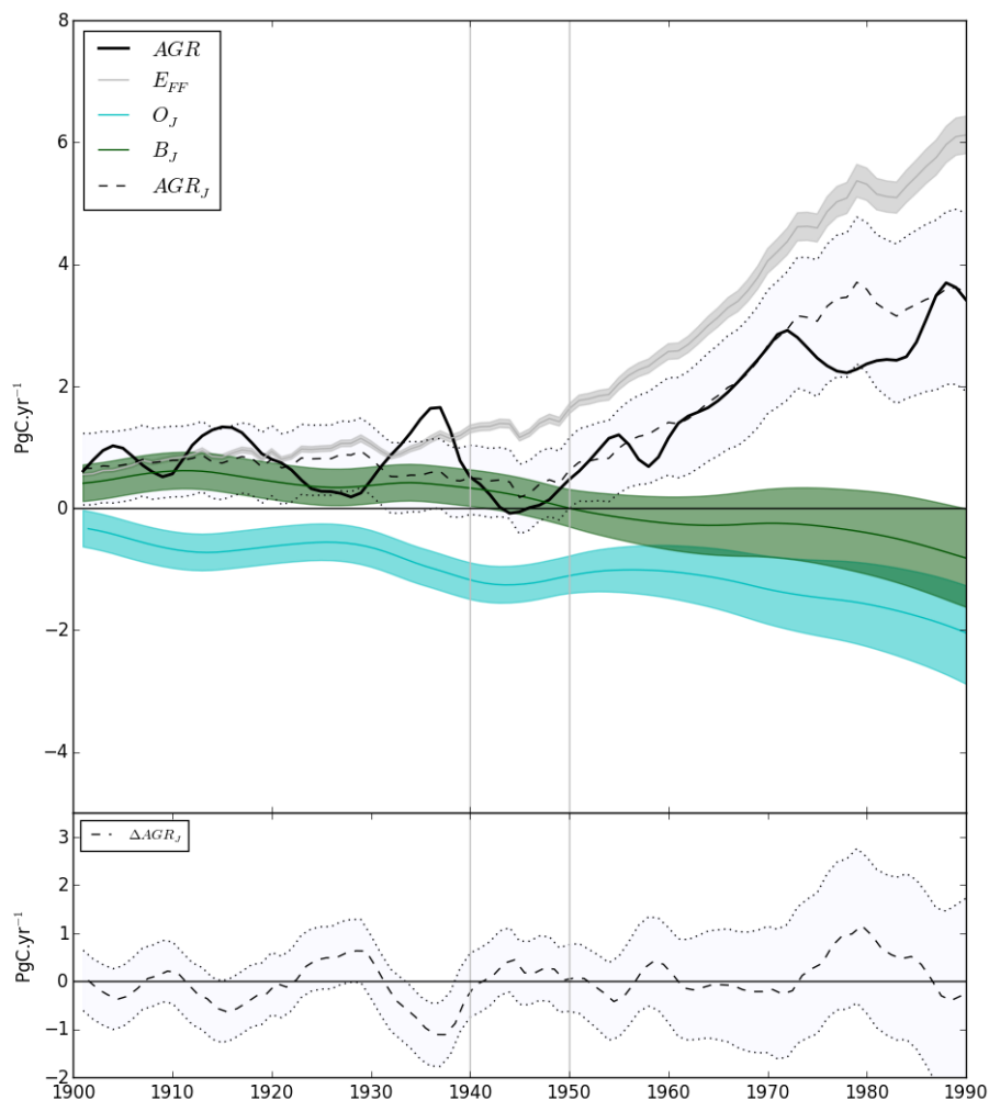
Figure 2. Atmospheric CO 2 growth rate (AGR) from the observational record, calculated from the spline fit in Figure 1 (black line, top panel). Fossil fuel emissions from the CDIAC database and respective uncertainty ( E_{FF} ), and the reconstruction of ocean and biospheric fluxes from Joos et al. (1999), O_J and B_J respectively (filled areas in top panel). The resulting balance from the latter three datasets ( AGR_J ) and uncertainty is shown in the top panel (dashed and dotted lines, respectively), and the corresponding difference between AGR and AGR_J is shown in the bottom panel.
