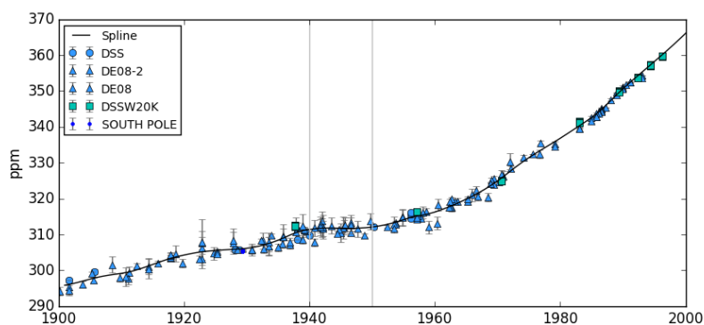
Figure 1. Atmospheric CO_2 concentration in the Law Dome ice core and firm record from Rubino et al. (2013) and respective uncertainties (markers and whiskers), and the spline-fit applied to the data following Enting et al. (2006), which attenuates by 50% variations of c.a. 23 years. The period corresponding to the plateau is highlighted between vertical grey lines.
