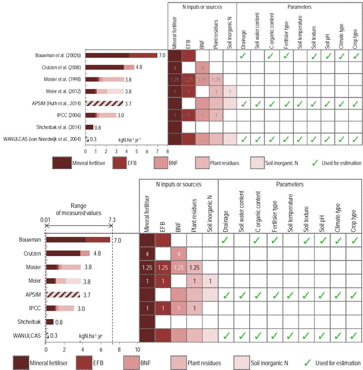
Figure 7. Comparison of annual average losses through N 2 O emissions, estimated by 8 sub-models. The average estimate was 3.4 kgN.ha -1 .yr -1 , ranging from 0.3 to 7 kgN.ha -1 .yr -1 . For APSIM, all sources are considered in one calculation. Measured values are from Pardon et al. (2016). The table shows the N inputs and parameters used by the sub-models, and emission factors for linear relationships. Emission factors are in % of N inputs. BNF: biological N fixation; EFB: empty fruit bunches, i.e. organic fertiliser.
