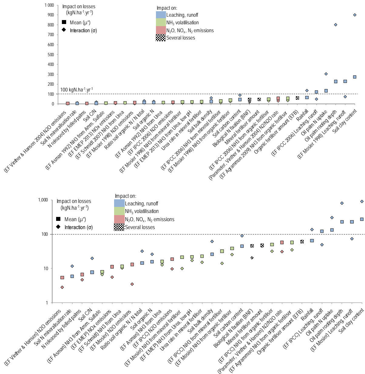
Figure 12. Average Morris indices for 31 variables of the 19 sub-models. The five variables having the highest influence ( \mu^* > 100 \text{ kgN.ha}^{-1}.\text{yr}^{-1} ) were related with leaching and runoff losses ( logarithmic scale ). Variables were ranked by increasing mean sensitivity index ( \mu^* ). The mean effect ( \mu^* , squares) was an estimation of the linear influence of the variable on losses. The interaction effect ( \sigma , diamonds) was an estimation of non-linear and/or interaction effect(s) of the variable on losses. Variables with \mu^* < 5 \text{ kgN.ha}^{-1}.\text{yr}^{-1} , i.e. 16 variables, are not represented. EF: emission factor; BNF: biological N fixation; EFB: empty fruit bunches, i.e. organic fertiliser.
