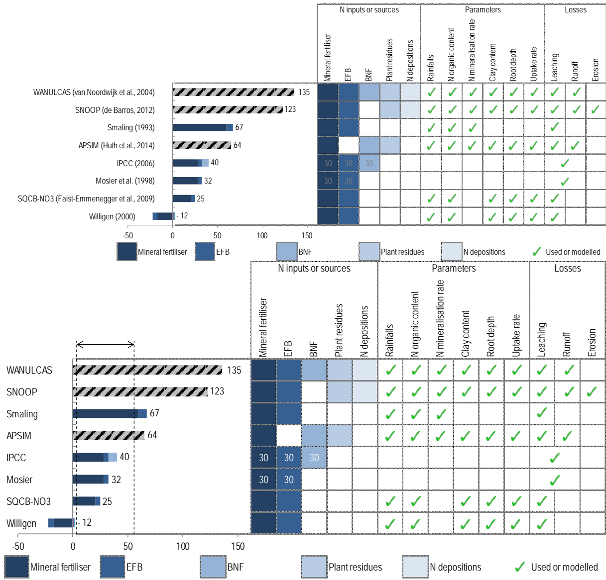
Figure 3. Comparison of annual average losses through leaching and runoff, estimated by 8 sub-models.
