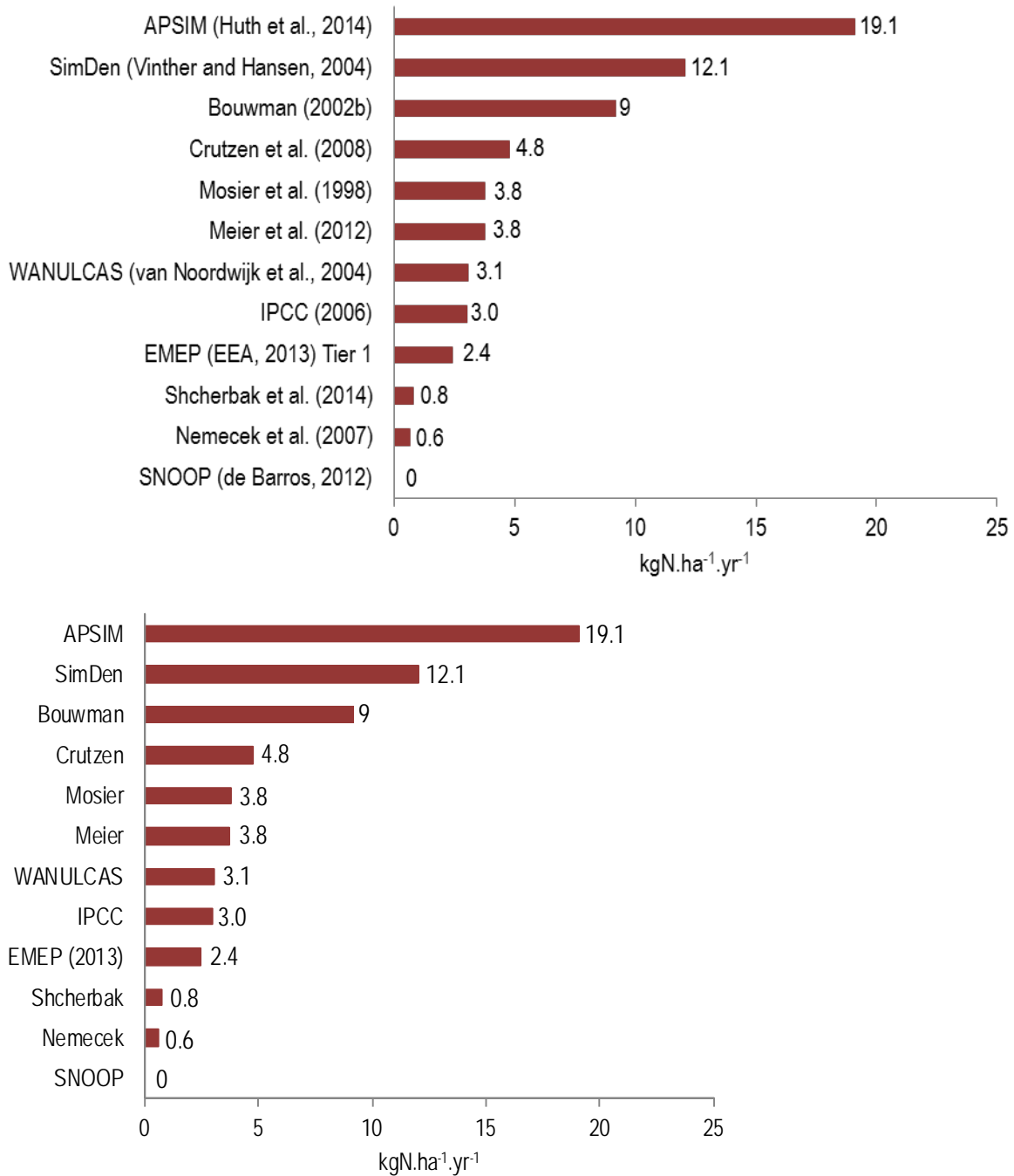
Figure 6. Comparison of annual average losses through N 2 O, N 2 , NO x emissions, estimated by 12 sub-models. The average estimate of combined N 2 , N 2 O and NO x emissions was 5.2 kgN.ha -1 .yr -1 . The wide range of 0 to 19.1 kgN.ha -1 .yr -1 could be explained partly because some sub-models estimated only N 2 O or NO x , while others calculated two or three of these gases jointly.
