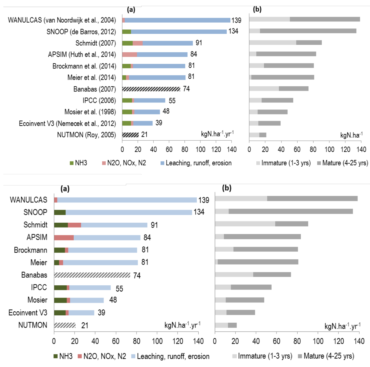
Figure 1. Estimates of N losses by 11 models. (a) Distribution of the annual average losses between the 3 pathways: leaching and runoff; NH 3 volatilisation; N 2 O, NO x , N 2 emissions. Overall losses of N were very variable, with an average of 77 kg N.ha -1 .yr -1 , ranging from 21 to 139 kg N.ha -1 .yr -1 . The leaching and runoff pathway was the most important of the three, corresponding to about 80% of the losses. The hatched bars represent calculations including several pathways at once: Banabas estimated jointly the 3 pathways, NUTMON estimated jointly all gaseous emissions and leaching losses were negative. SNOOP estimated N 2 , N 2 O, and NO x emissions as null, and APSIM and WANULCAS did not model the NH 3 volatilisation. (b) Distribution of the annual average losses between the immature and the mature phases, corresponding to 1-3 years, and 4-25 years after planting; respectively. On average, 31% of the losses occurred during the immature period, which represents 12% of the cycle duration.
