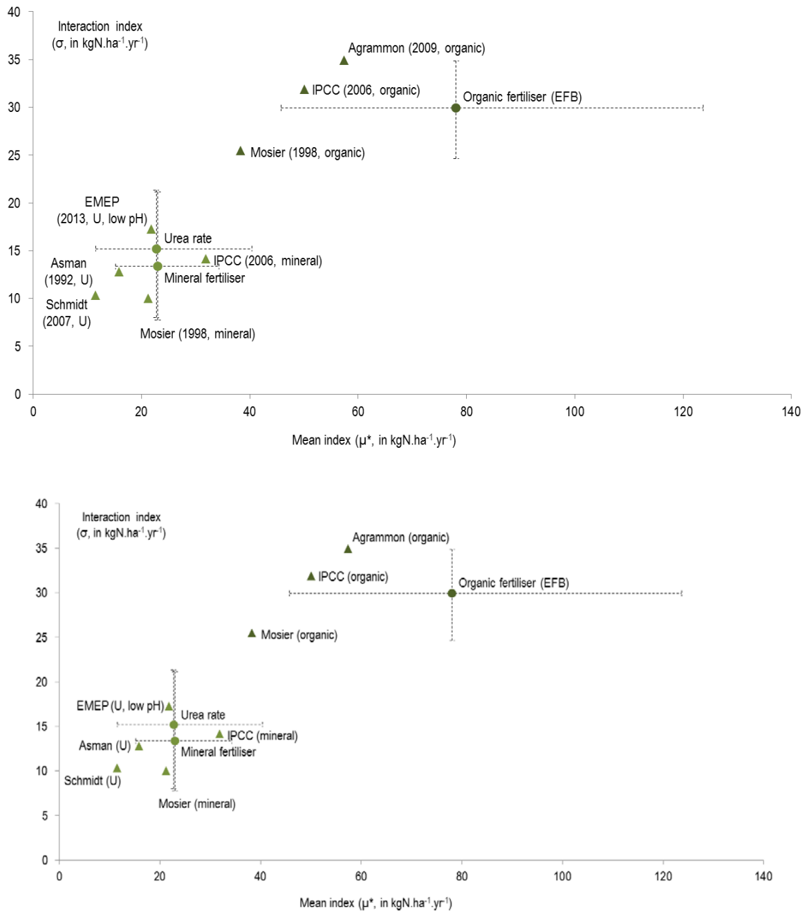
Figure 10. Morris's sensitivity indices for sub-models calculating NH 3 volatilisation. The input variables related with organic inputs (dark green) had higher Morris indices than mineral inputs (clear green). Sub-models tested: IPCC 2006, Mosier, Asman, Schmidt, Agrammon, EMEP 2009 and EMEP 2013. Indices lower than 10 kgN.ha -1 .yr -1 are not represented. Triangles: emission factors; circles: N inputs. AS: Ammonium Sulfate; U: Urea; EFB: empty fruit bunches, i.e. organic fertiliser.
