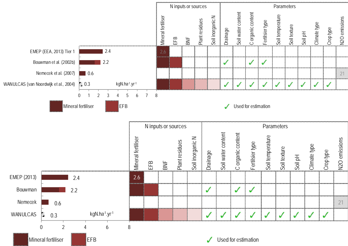
Figure 8. Comparison of annual average losses through \text{NO}_x emissions, estimated by 4 sub-models sub-models. The average estimate was 1.4 \text{ kgN.ha}^{-1}.\text{yr}^{-1} , ranging from 0.3 to 2.4 \text{ kgN.ha}^{-1}.\text{yr}^{-1} . For Nemecek 2007, all sources are considered in one calculation. The table shows the N inputs and parameters used by the sub-models, and emission factors for linear relationships. Emission factors are in % of N inputs. EFB: empty fruit bunches, i.e. organic fertiliser.
