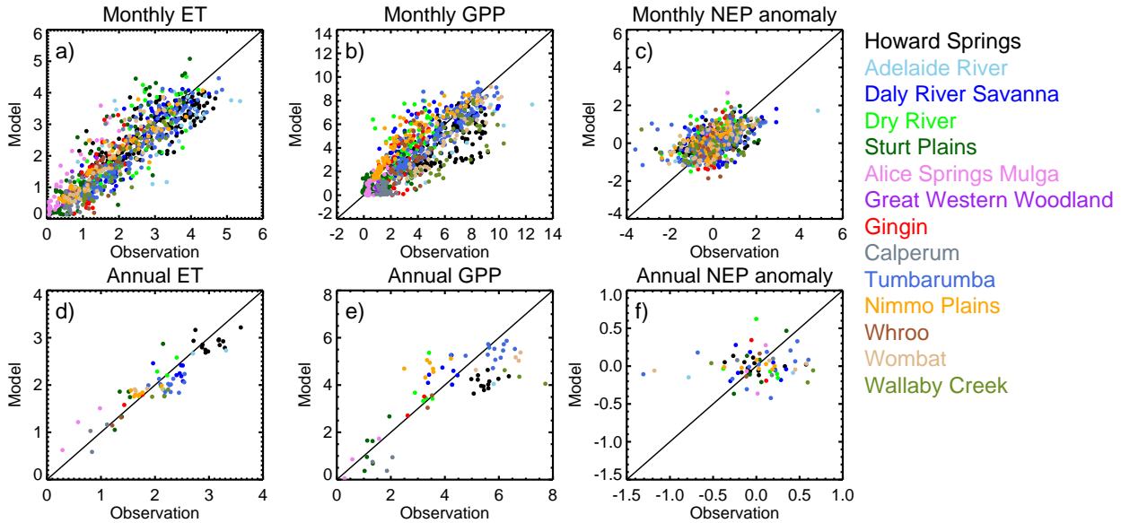
Figure 5. Scatter plots of observed and modelled (best case) monthly and annual ET ( \text{mm d}^{-1} ), GPP ( \text{gC m}^{-2} \text{d}^{-1} ) and NEP ( \text{gC m}^{-2} \text{d}^{-1} ) at 14 Ozflux sites. Symbols are color-coded according to site.
