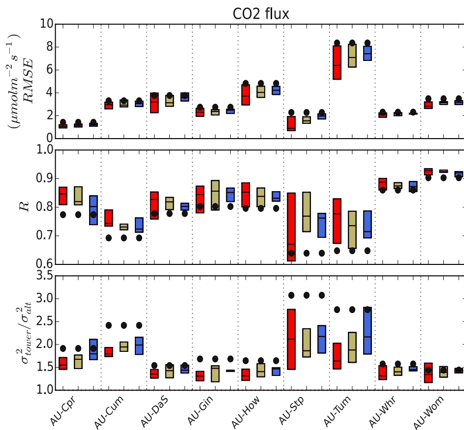
Figure 6: Statistics for different gap filling window lengths for CO 2 flux. Window lengths are 60 days (red), 182 days (green), 365 (blue) and the whole length of the data set (black dots). Box lengths represent the 75% and 25% quartiles with the median plotted across the boxes as a solid line.
