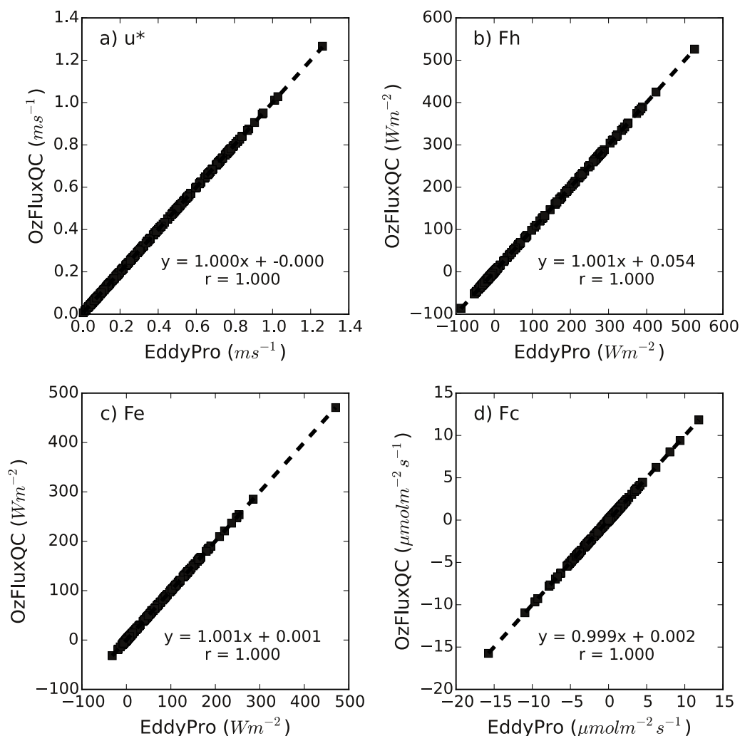
Figure 8: Comparison of friction velocity ( u^* ), sensible heat flux ( F_h ), latent heat flux ( F_e ) and CO_2 flux ( F_c ) calculated using EddyPro and OzFluxQC. Data are from the AU-How site for the period 2011/06/09 to 2011/08/05.
