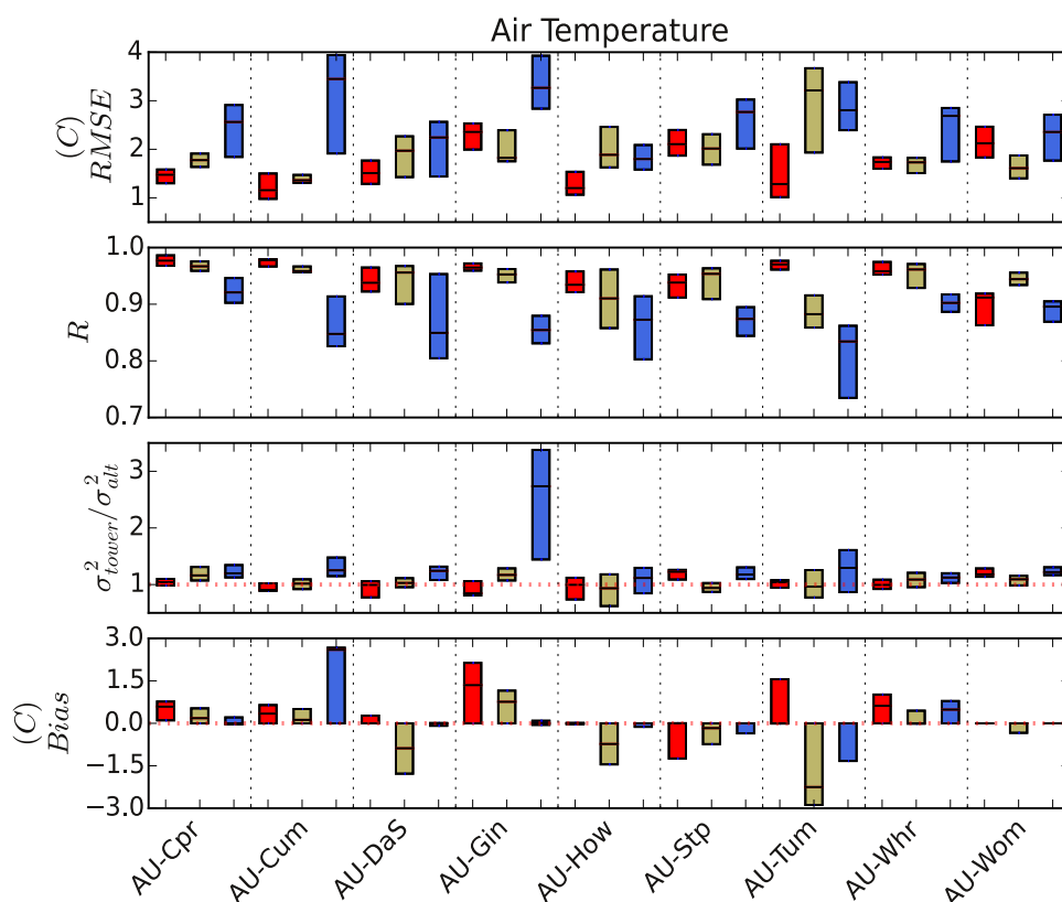
Figure 5: Box plot of bias, variance ratio, correlation coefficient and root mean square error for the comparison of tower and alternate air temperature at 9 OzFlux sites. Statistics for AWS are plotted in red, ACCESS-R in green and ERA Interim in blue. Box lengths represent the 75% and 25% quartiles and the median is plotted as a solid line across the boxes.
