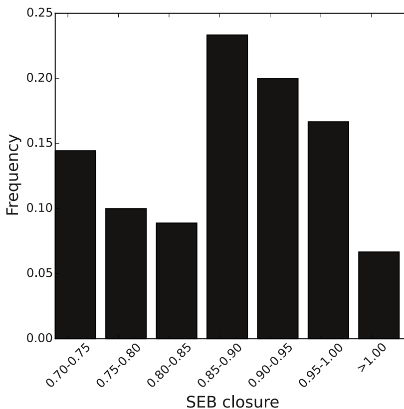
Figure 7: Histogram of surface energy balance closure for 86 site-years of data across 23 sites.
