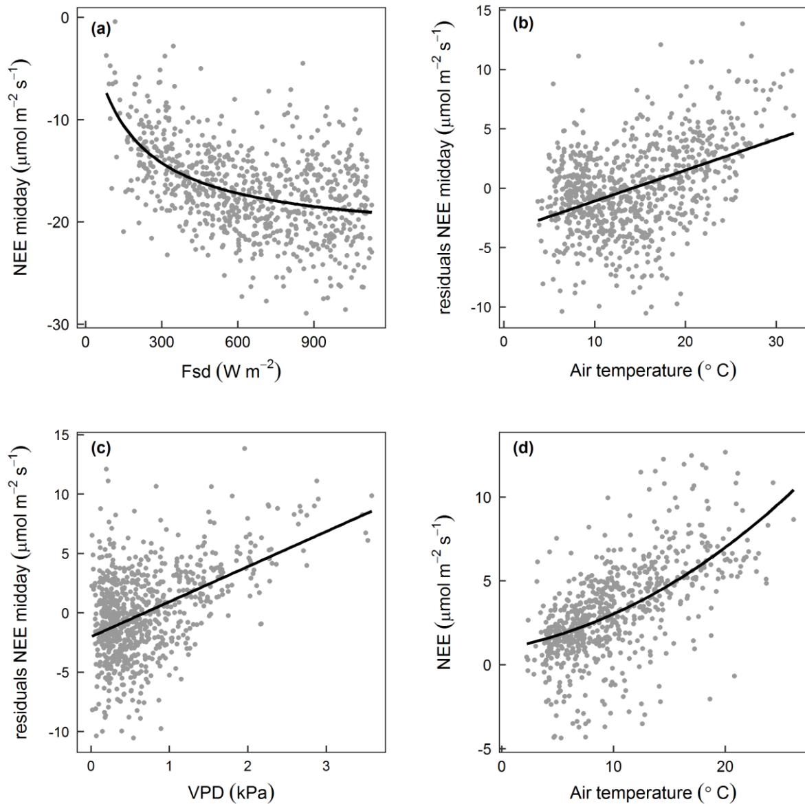
Figure 5: (a-c) Relationship between daily means of midday NEE and (a) incoming solar radiation (Fsd) as a rectangular hyperbolic light response curve (LRC), linear fits between residuals of LRC and (b) air temperature ( T_a ) or (c) vapour pressure deficit (VPD) and (d) relationship between daily means of u^* filtered night time NEE and air temperature as temperature ( T_a ) response function after Lloyd and Taylor (1994), R^2 are given in Table 3 and 5.
