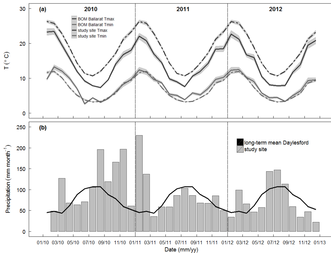
805 Figure 1: Climate time series of (a) monthly averages of minimum (grey lines) and maximum (black lines) air temperatures from the study site from 2010 to 2012 (solid lines) and from the BoM station Ballarat from 2001 to 2013 (dashed lines), shaded areas indicate \pm 1SE , and (b) monthly rainfall at Wombat State Forest OzFlux EC tower site from 2010 to 2012 (grey bars) and 114 year (1901-2014) long-term monthly mean rainfall at BoM station Daylesford (black line)
