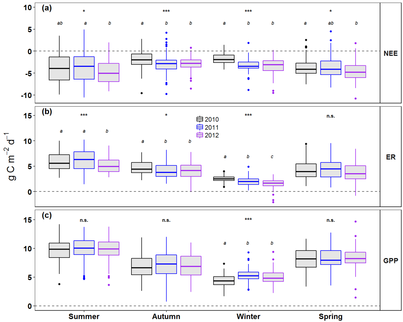
Figure 4: Box- and whisker plots of daily averages of a) NEE, b) ER and c) GPP for years and seasons; inter-annual differences are displayed for each seasons with p-values (significance level p < 0.05 ), letters indicate year to year differences
