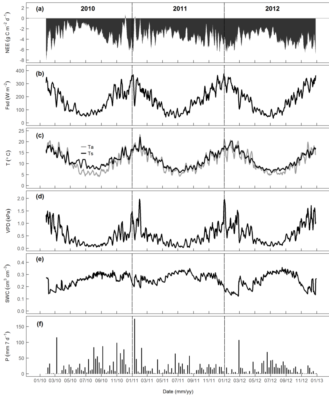
Figure 2: Time series of (a) 7-day running means of daily total net ecosystem exchange (NEE), 7-day running means of daily averages of (b) incoming solar radiation (Fsd), (c) air (Ta) and soil (Ts) temperature, and (d) 7-day running means of mean midday (11:00-13:00) vapour pressure deficit (VPD), (e) daily averages of volumetric soil water content (SWC) and (f) 7-day sums of rainfall (P) from 2010 to 2012
