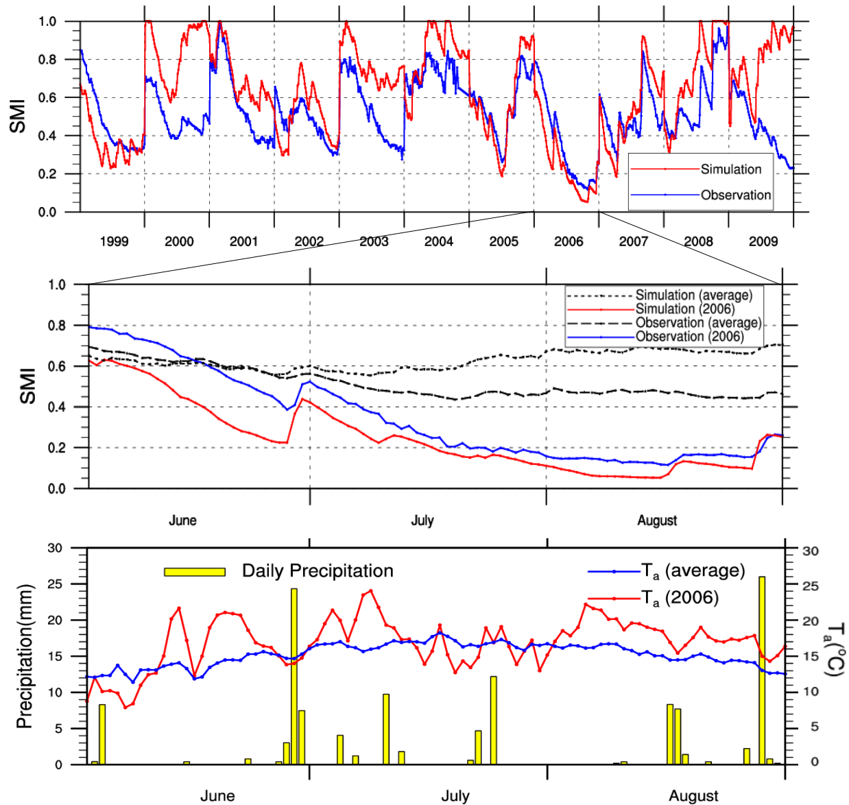
540 Figure 1: (a) Daily mean soil moisture index (SMI) at Hyttiälä from observation and the JSBACH simulation for the summer months (June, July, August) in the 11-year study period (from 1999 to 2009). (b) Daily mean SMI at Hyttiälä from observation and the JSBACH simulation for the summer months in 2006; The two black dashed lines represent the averaged daily SMI in the summer months over the 11-year study period from observation and the JSBACH simulation. (c) Daily mean air temperature ( T_a ) in the summer months of 2006 and the averaged 545 daily mean T_a in the summer months over the 11-year study period at Hyttiälä from observation, meanwhile, the daily precipitation amount in 2006 is shown as bar plot.
