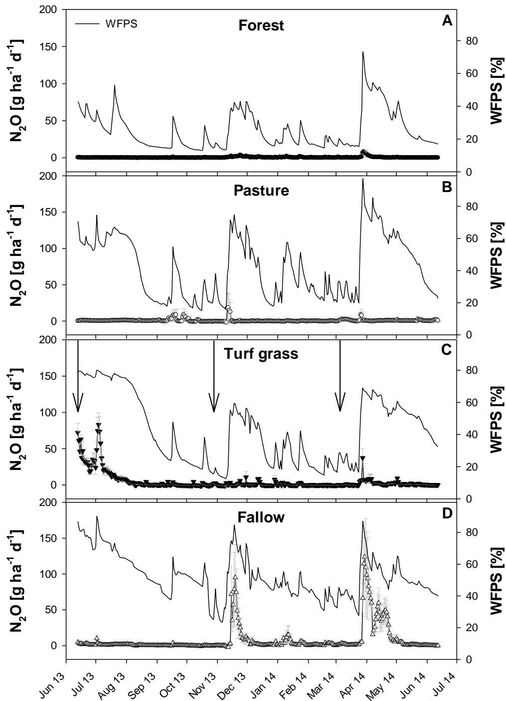
Figure 2: Daily N_2O flux averages (max 8 fluxes per day for 3 replicates each) with standard errors ( n = 3 ) over the experimental year 2013/2014 for forest (A), pasture (B), turf grass (C) and fallow (D) with the treatment specific water filled pore space (WFPS).
