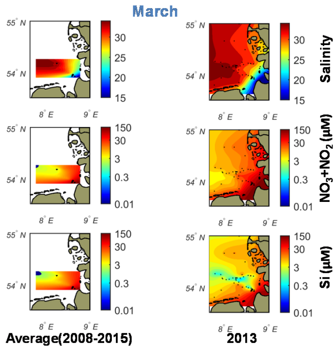
Fig. 10: Maps of interpolated (Kriging method of interpolation) salinity, nitrate + nitrite ( \text{NO}_3 + \text{NO}_2 ( \mu\text{M} )), and silicate ( \text{Si} ( \mu\text{M} )) for the month of March. The left panels show average parameter distributions in March, based on 7 years of data (2008-2015, excluding 2013) from BAH AWI stations (Table 1); the right panels show interpolated parameters from 15 to 27 March, 2013 from 2013, measured at BAH AWI, BSH, FerryBox and HPA stations (Table 1 and 4), were sampled between 15 and 27 March, 2013.
