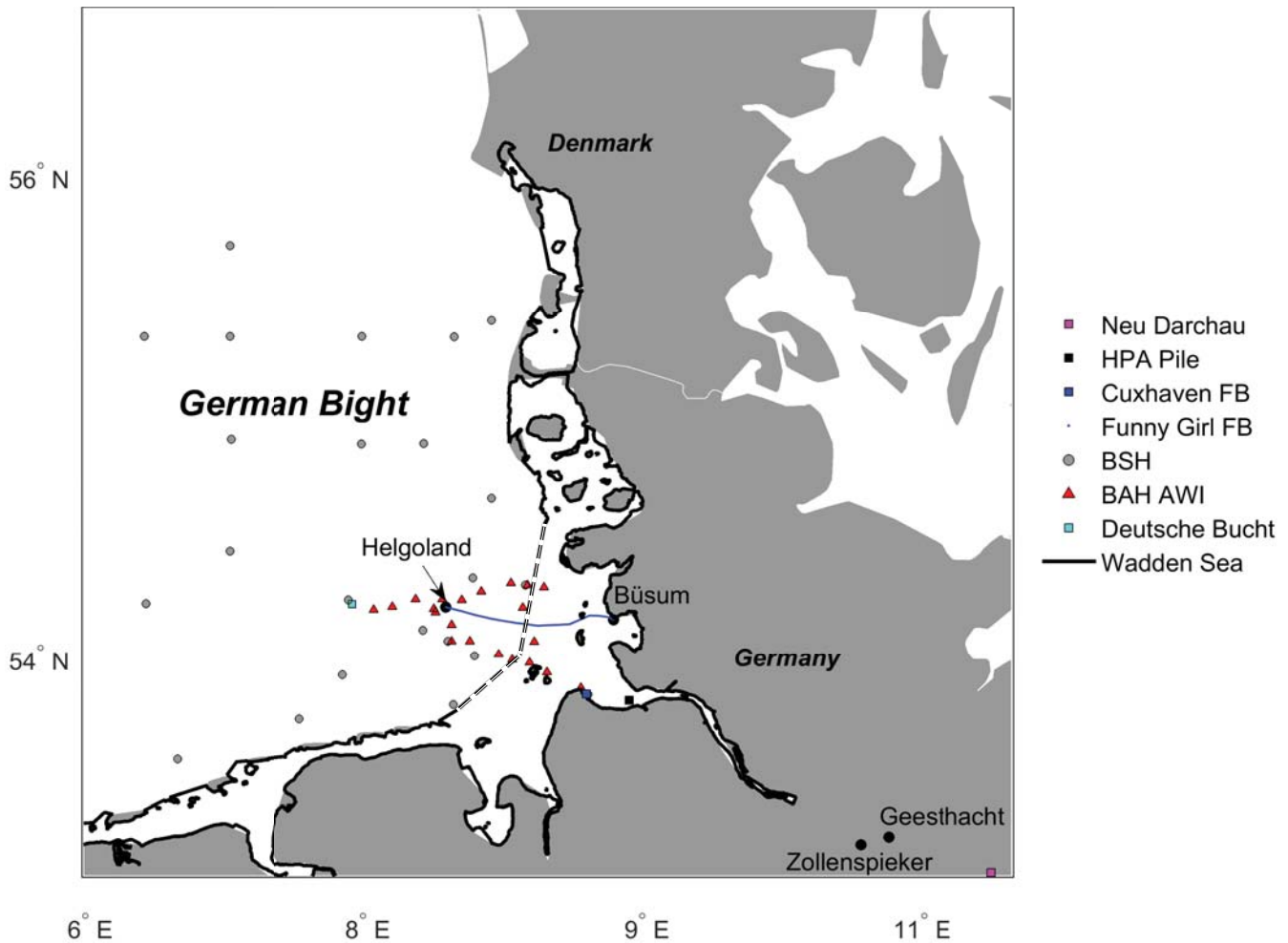
5 Fig. 1: Map of German Bight, Elbe Estuary, Wadden Sea and the continental regions around them. Stations are indicated with different symbols. Neu Darchau discharge gauging station (magenta square), operated by the German Federal Waterways and Shipping Administration (WSV); HPA Pile (black square), operated by Bundesamt für Seeschifffahrt und Hydrographie (BSH) and Helmholtz-Zentrum Geesthacht (HZG); Cuxhaven FerryBox (FB, blue square), operated by HZG, M/V Funny Girl FB transect (blue line) between Büsum and Helgoland, operated by HZG; BSH discrete sampling stations (grey circles); Biological Station Helgoland at the Alfred Wegener Institute (BAH AWI) discrete sampling stations (red triangles); Deutsche Bucht MARNET monitoring station, operated by BSH (cyan square). The Wadden Sea outline was obtained as a shape file from Claus et al. (2016), and the dashed line represents the imaginary 10 boundary of the shapefile, rather than the Wadden Sea.
