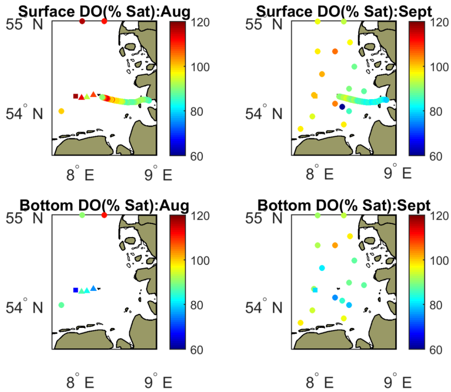
Fig. 14: Dissolved oxygen (% saturation) in surface and bottom waters measured in August and September, 2013 meteorological meteorology. The surface and bottom dissolved oxygen were measured at available discrete stations from AWI and BSH stations, along with FerryBox (M/V Funny Girl ) and Deutsche Bucht MARNET station. The dates of coverage are listed in Table 4.
