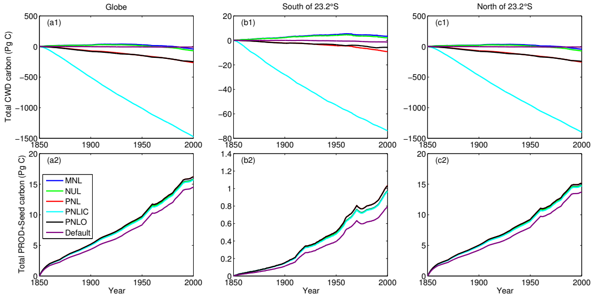
Figure S3: (a1), (b1) and (c1) are carbon changes in total coarse woody debris. (a2), (b2) and (c2) are changes in total product carbon and seed carbon.
