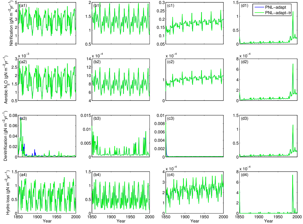
Figure S9: Evaluation of the ordering effect for the point simulations. PNL-adapt-tr simulates transports ahead of biogeochemical calculations, whereas PNL-adapt does the opposite order. From left to right, the four columns are representing sites that are corresponding to the locations specified in Figure 3 of the main text.
