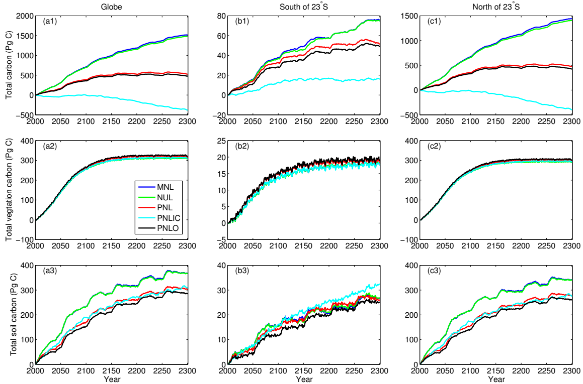
Figure S6: Model simulations for the scenario Representative Concentration Pathway 4.5 (RCP4.5) atmospheric CO 2 for the years 2001-2300. Here total soil carbon includes litter carbon and soil organic matter as defined in CLM4.5; coarse woody debris is excluded. All changes are calculated as relative to each of their initial carbon pool sizes at the start of the simulation (i.e. end of year 2000). The oscillations as shown in the figure are due to the cycling of the QIAN climate forcing.
