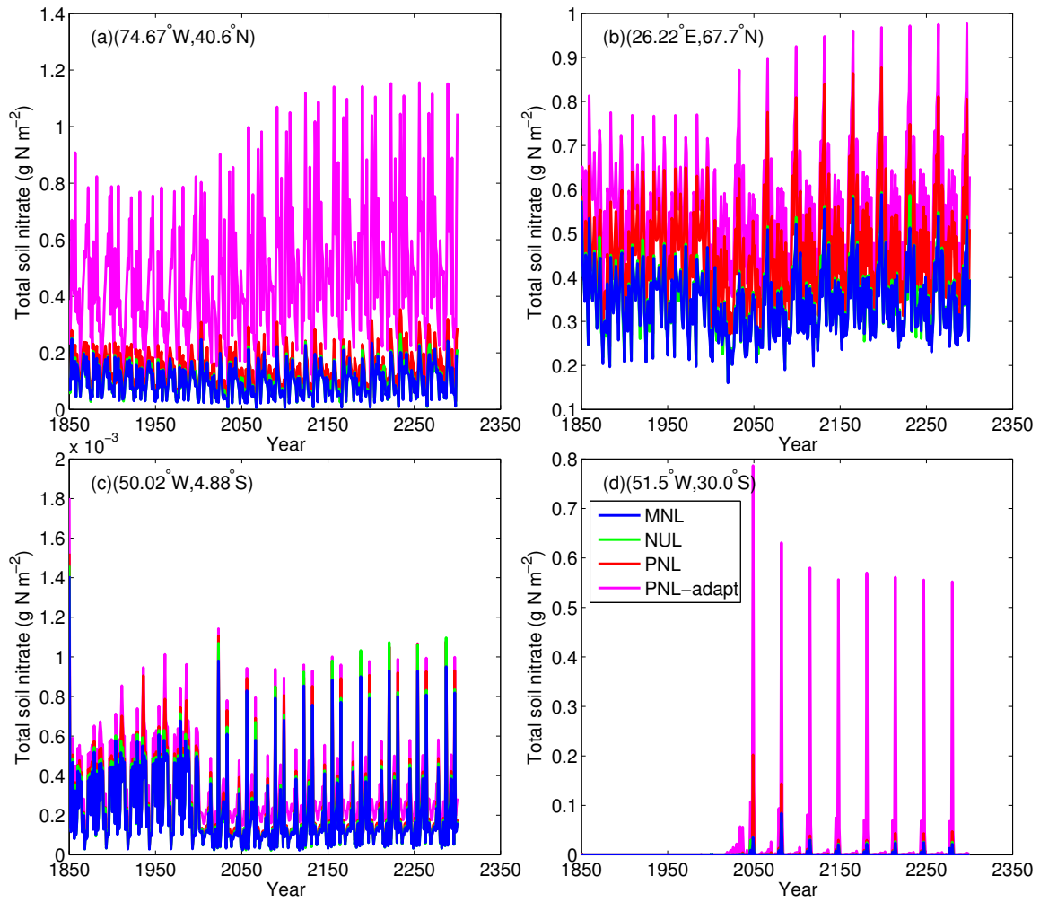
Figure S10: Soil nitrate concentrations for the point simulations as obtained from different model configurations.
