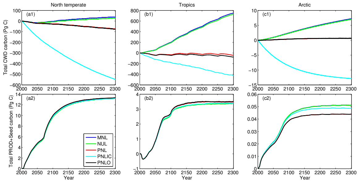
Figure S7: Simulated evolution of coarse woody debris carbon (a1-c1) and product and seed carbon (a2-c2) for the RCP 4.5 CO 2 driven period 2001-2300. These results are complementary to Figure 2 in the main text.
