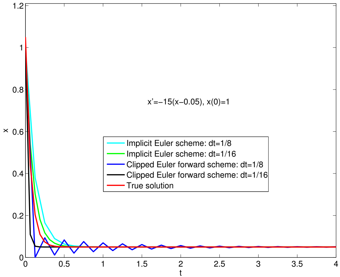
Figure S11: A demonstration of the zigzag phenomena and the strong time-stepping dependence of the numerical solution using Euler methods.
