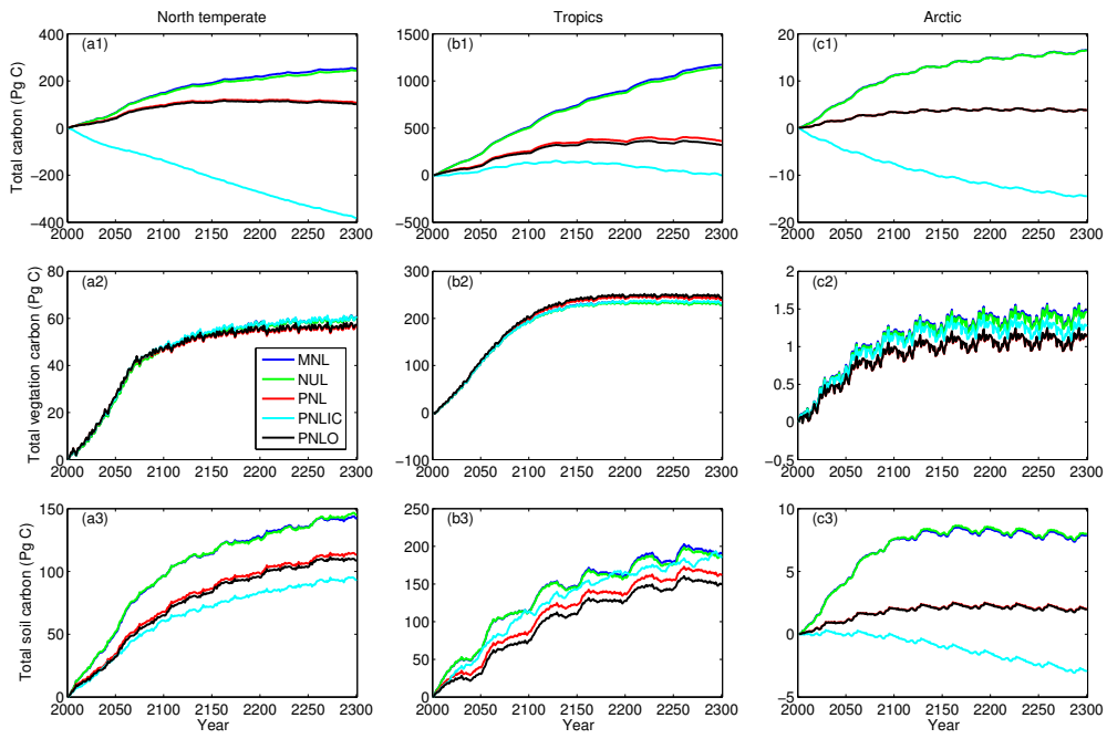
Figure 2. Model simulations forced by the Representative Concentration Pathway 4.5 (RCP4.5) atmospheric CO 2 for year 2001-2300. Here total soil carbon includes litter carbon and soil organic matter as defined in CLM4.5 (Oleson et al., 2013); coarse woody debris is excluded (but can be found in Figure S7). All changes are calculated as relative to each of their initial carbon pool sizes at the start of the simulation (year 2000). The decadal oscillation shown in the figure is due to the cycling of the QIAN climate forcing.
