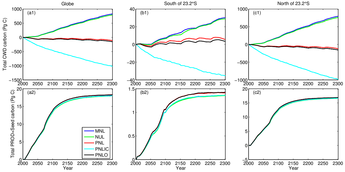
Figure S8: Simulated evolution of coarse woody debris carbon (a1-c1) and product and seed carbon (a2-c2) for the RCP 4.5 CO 2 driven period 2001-2300. These results are complementary to Figure S6 above.
