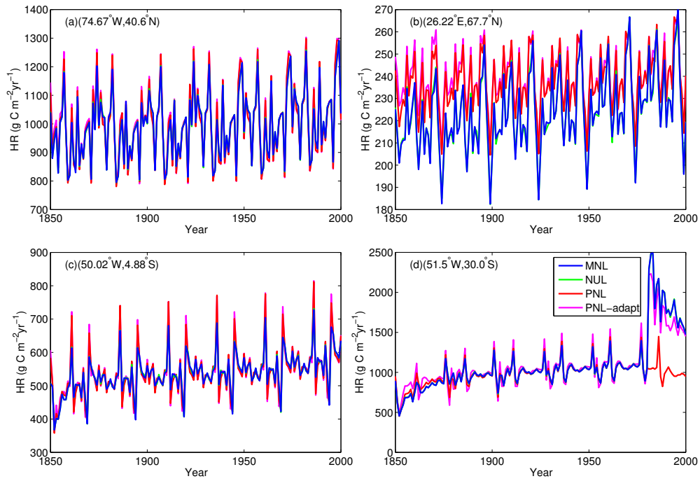
5 Figure 5. Heterotrophic respiration for the four specific gridcell simulations obtained from running different model configurations. The decadal oscillation shown in the figure is due to the cycling of the QIAN climate forcing.
