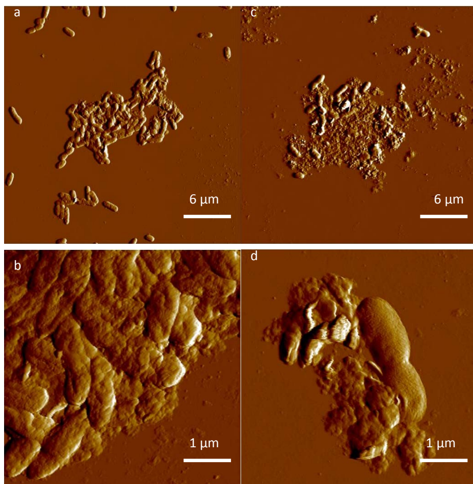
Figure S2. AFM image of montmorillonite- B.subtilis composite at pH 3.0 (a, b) and pH 7.85 (c, d, ). Morphology measurements of the composite was followed the procedure outlined by Huang et al. (2015).
