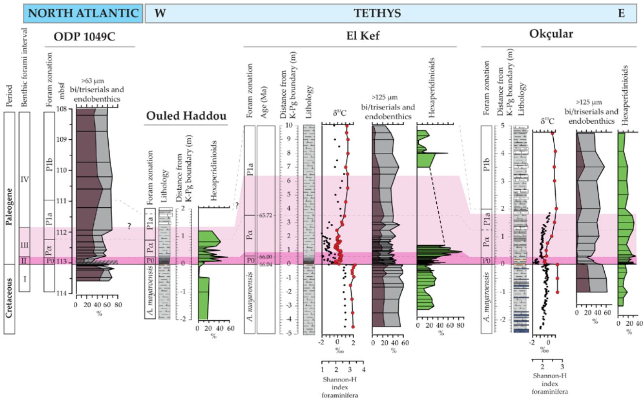
Figure 8: The benthic foraminiferal (>125 \mu m), dinocyst and bulk stable carbon isotope records of Okçular (Turkey) and El Kef (Tunisia), the dinocyst record of Ouled Haddou (Morocco) and the benthic foraminiferal record (>63 \mu m) of ODP 1049C Blake Nose (North Atlantic). Note that the definition of ‘hexaperidinioids’ used is provided in the text. The 4 phases identified based on the bulk stable carbon isotopes and the Shannon-H index of the benthic foraminiferal records, are indicated (I-IV). The >63 \mu m size fraction benthic foraminiferal record of ODP 1049C is from Alegret and Thomas (2004), who argued that the lowermost Paleocene of this site comprised reworked foraminifera. This interval is indicated by a dashed bar in the figure. The biostratigraphy of Ouled Haddou is from Slimani and Toufiq (2013), whereas the dinocyst record of this site is from Slimani et al. (2010). The biostratigraphy of El Kef is based on Brinkhuis et al. (1998), Speijer and van der Zwaan (1996) and Molina et al. (2006). The fine fraction bulk stable carbon isotope record (black dots) of El Kef is from Keller and Lindinger (1989). The Shannon-H index (red dots) and relative abundances of bi-/triserial benthic taxa (dark purple) and all endobenthic foraminifera (light purple) are based on the >125 \mu m size fraction foraminiferal data of Speijer and van der Zwaan (1996). The palynological data of El Kef is from Brinkhuis et al. (1998) (lower part) and Guasti et al. (2005) (upper part). The Shannon-H index of the >125 \mu m size fraction benthic foraminiferal record (red dots), the relative contribution of bi-/triserial benthic taxa (dark purple), all endobenthic foraminifera (light purple) and hexaperidinioid dinocysts from Okçular are from this study. The bulk stable carbon isotope record of Okçular (black dots) is from Açıkalın et al. (2015). Mbsf=meters below sea floor.
