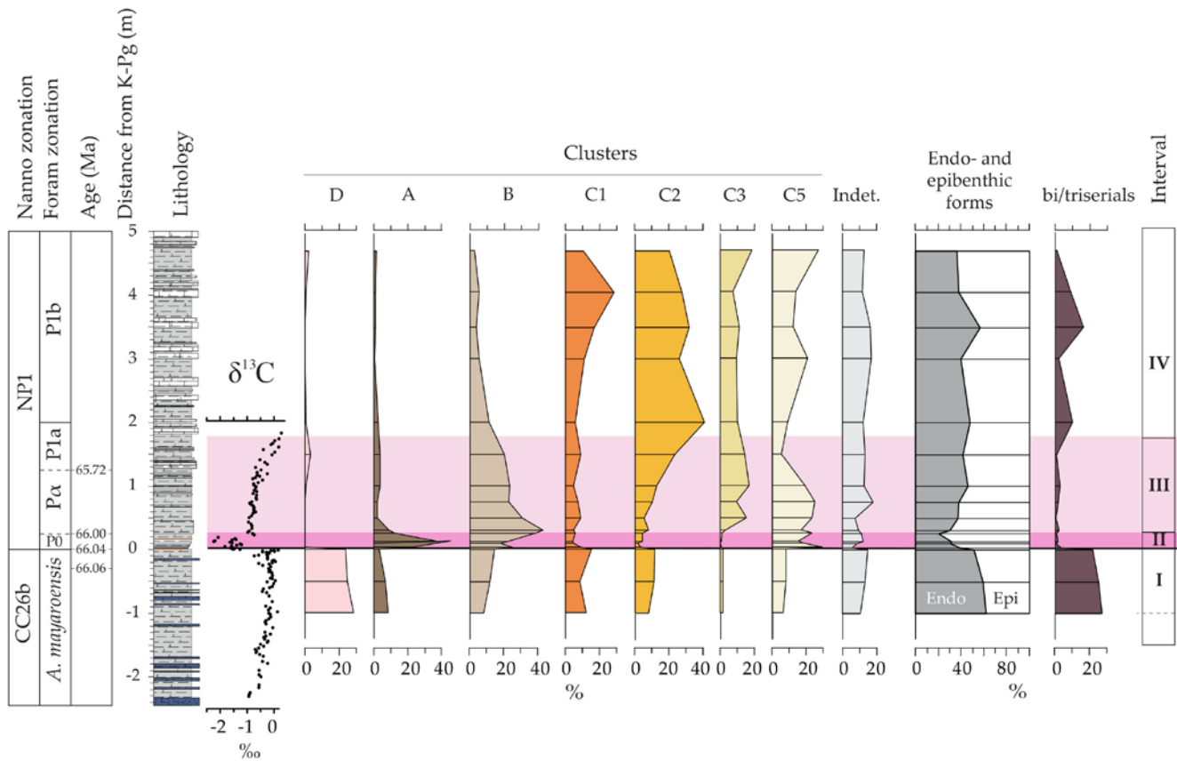
Figure 6: Relative abundances of the 4 main clusters of benthic foraminiferal taxa (>125 \mu\text{m} ), relative abundances of epibenthic and endobenthic forms and relative abundance of bi-/triserial benthic taxa.
