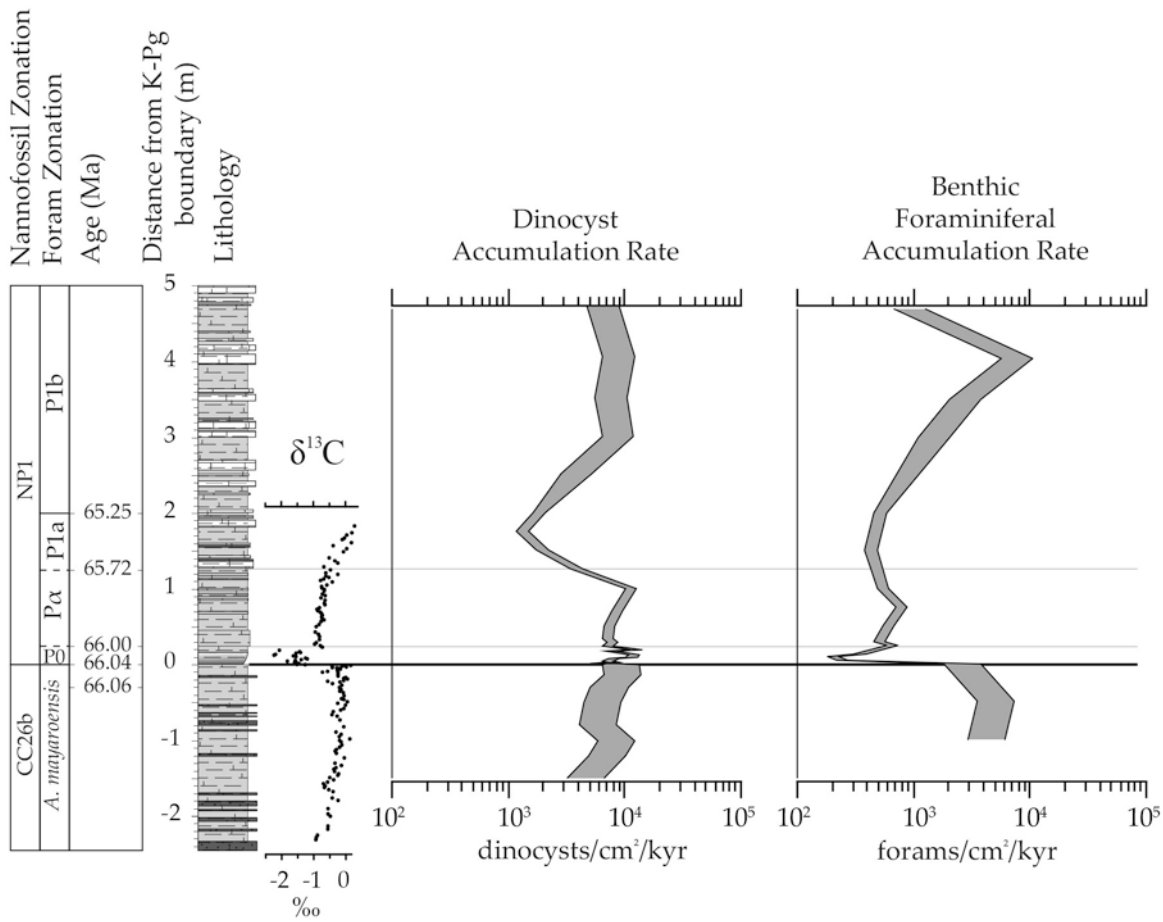
5 Figure 5: Estimated Benthic Foraminiferal Accumulation Rate (BFAR; number of foraminifera of the >63 \mu\text{m} size fraction per cm 2 sea floor per kyr) and estimated Dinocyst Accumulation Rate (DAR; number of preserved cysts per cm 2 sea floor per kyr) of the Okçular section. Uncertainty in estimated accumulation rates, resulting from uncertainties in sediment densities and sedimentation rates, are indicated in grey, providing a range of estimated accumulation rates. For more detailed info on the calculation of the BFAR and DAR, see Text S2 of the supplementary online material.
