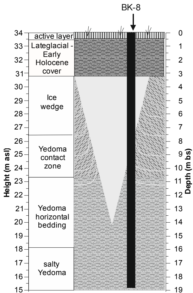
Figure 7. Scheme of the BK-8 permafrost core including the main cryolithological units. The legend is given in Figs. 4 and 6.
