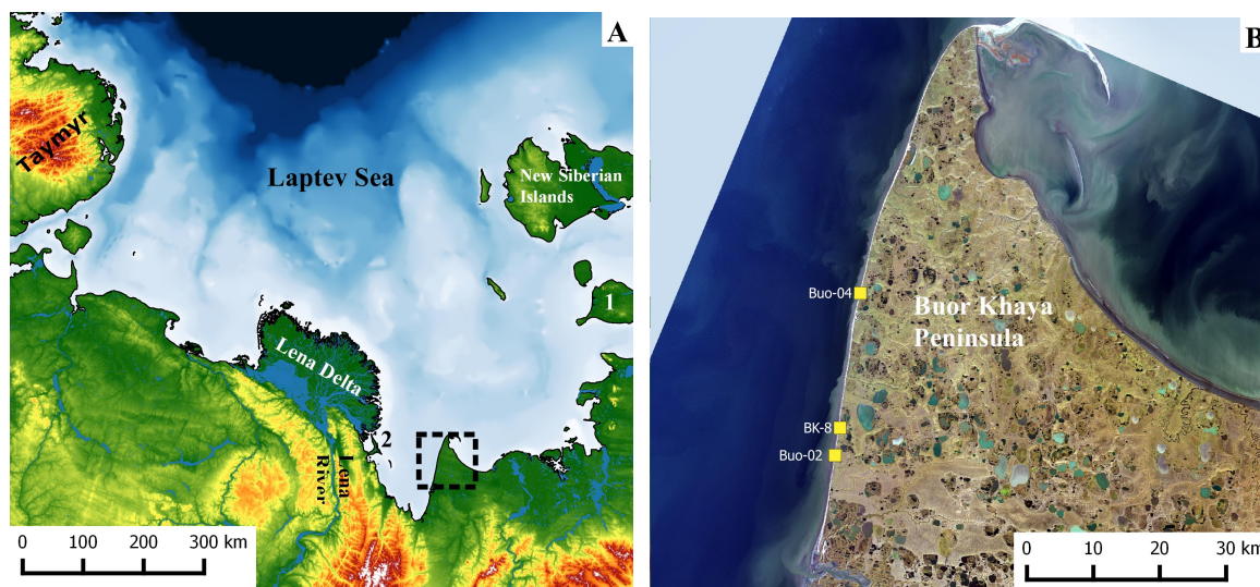
Figure 1. Study region in the central Laptev Sea (A, based on IBCAO 3.0 Jakobsson et al. 2012) including Buor Khaya Peninsula marked by the black frame and Yedomo IC reference sites on Boløshoy Lyakhovsky Island (1) and Bykovsky Peninsula (2); and position of the study sites Buo-02, Buo-04, and BK-8 at the western coast of the Buor Khaya Peninsula (B, LANDSAT_8 image from 2015).
