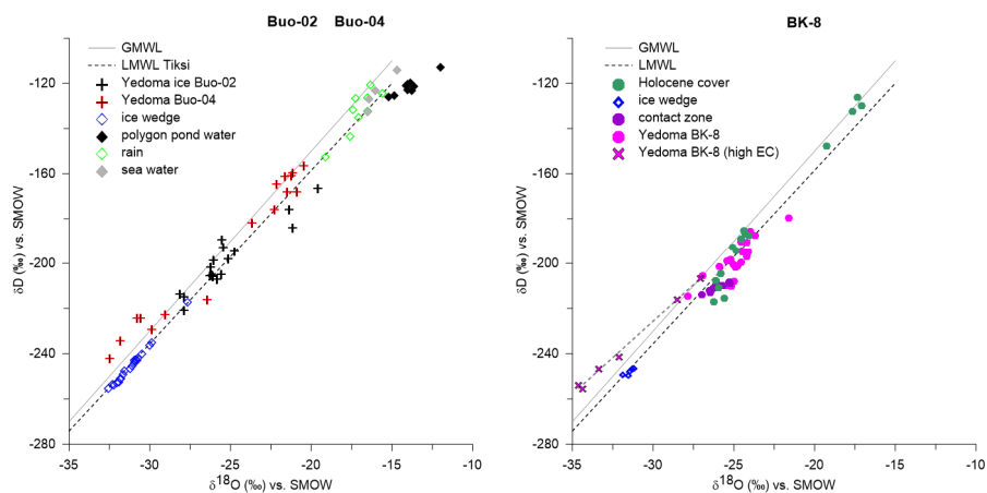
Figure 12. Stable isotope ratios for the Buoy-02 and Buoy-04 exposures and the BK-8 core samples. For reference, they are plotted together with precipitation and meteoric water lines, both global (GMWL; solid line) and local (LMWL; dashed line).
