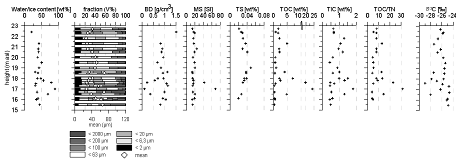
Figure 4. Cryolithological and organic matter properties of the Buo-02 profile (note that due to overlapping sub-profiles, different values may be displayed at similar heights).
