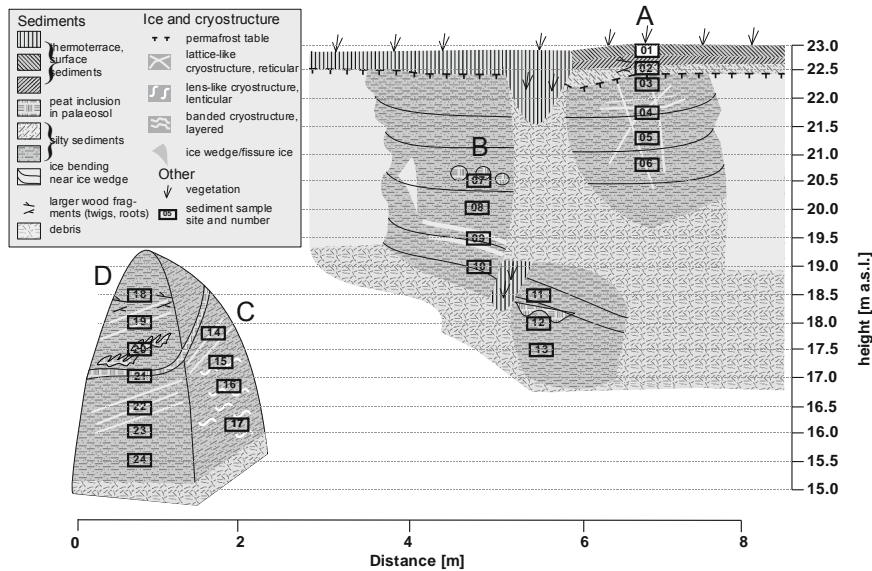
Figure 3. Overview photo and scheme of the Buo-02 Yedoma IC exposure with sample positions and main cryolithological features (modified from Strauss and Schirrmeister, 2011 ).
