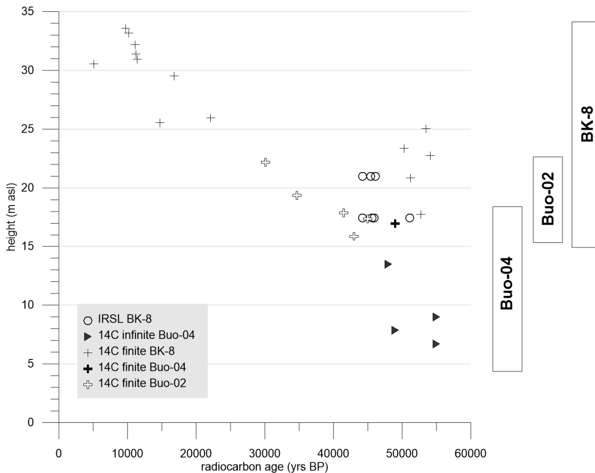
Figure 13. Compilation of geochronological results of Yedoma IC obtained in two profiles (Buo-02, Buo-04) and one drill core (BK-8) at the western coast of Buor Khaya Peninsula.
