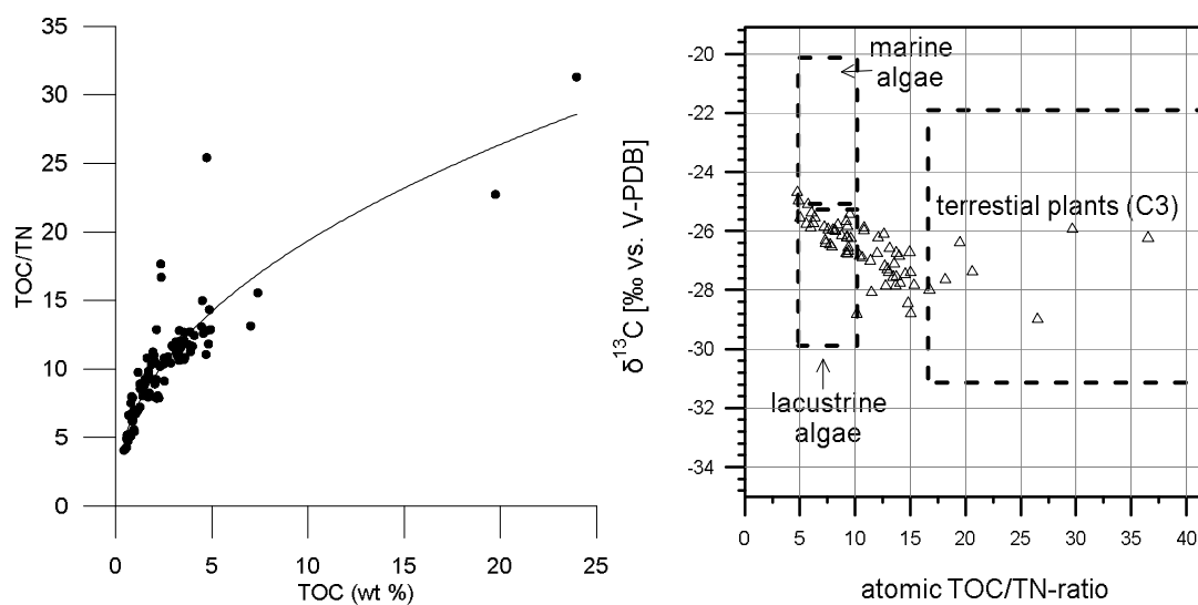
Figure 16. Organic matter characteristics of the Buor Khaya Yedoma. Left: Correlation of the TOC content and the TOC/TN ratio. Right: Distribution of the TOC \delta^{13}\text{C}_{\text{TOC}} relationships according to Meyers (1997).
