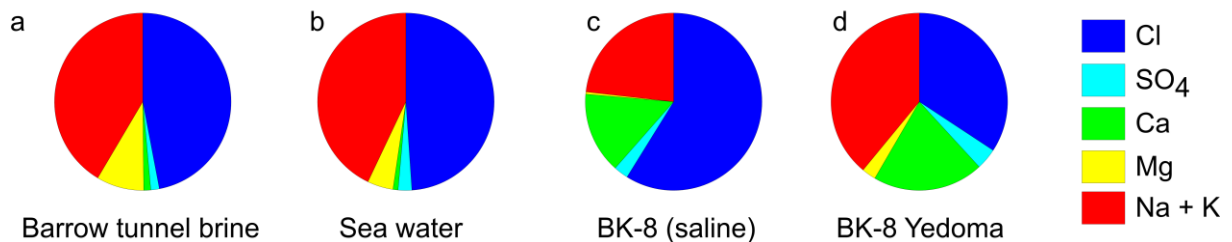
Figure 15. Comparison of major ion composition of a) saline brine from the Barrow permafrost tunnel in Alaska (Colangelo-Lillis et al., 2016), b) sea water with the pore water in the BK-8 Yedoma core from the lowermost saline layers (c) and the overlying Yedoma (d).
