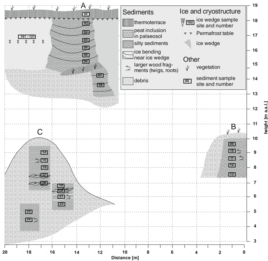
Figure 5. Overview photo and scheme of the Buo-04 Yedoma IC exposure with sample positions and main cryolithological features (modified from Strauss and Schirrmeyer, 2011).
