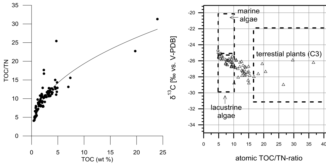
Figure 16. Organic matter characteristics of the Buor Khaya Yedoma. Left: Correlation of the TOC content and the TOC/TN ratio. Right: Distribution of the TOC – \delta^{13}\text{C}_{\text{TOC}} relationships according to Meyers (1997).
