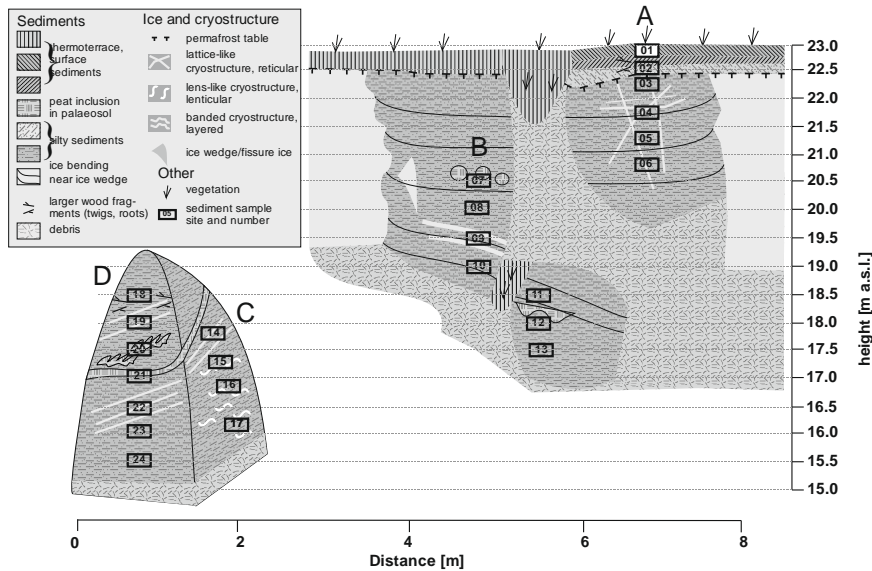
Figure 3. Overview photo and scheme of the Buoy-02 Yedoma IC exposure with sample positions and main cryolithological features (modified from Strauss and Schirrmeister, 2011).
