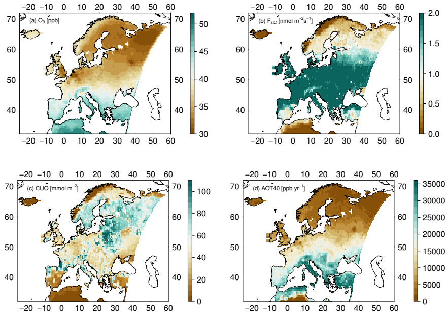
Figure 6. Mean decadal a) O_3 concentration [ppb], b) canopy integrated O_3 uptake into the leaves [ nmol\ m^{-2}\ s^{-1} ], c) canopy integrated cumulative uptake of O_3 (CUO) [ mmol\ m^{-2} ] and d) AOT40 [ ppb\ yr^{-1} ], for Europe of the years 2001-2010.
