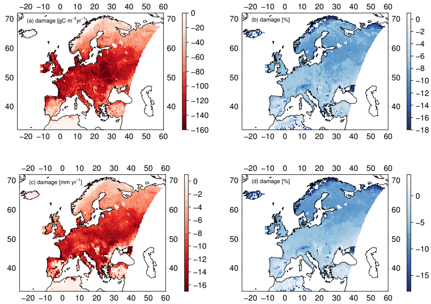
Figure 7. Mean decadal a) reduction in GPP [ g\ C\ m^{-2}\ yr^{-1} ], b) percent reduction in GPP, c) reduction in transpiration [ mm\ yr^{-1} ] and d) percent reduction in transpiration due to ozone damage averaged for the years 2001-2010.
