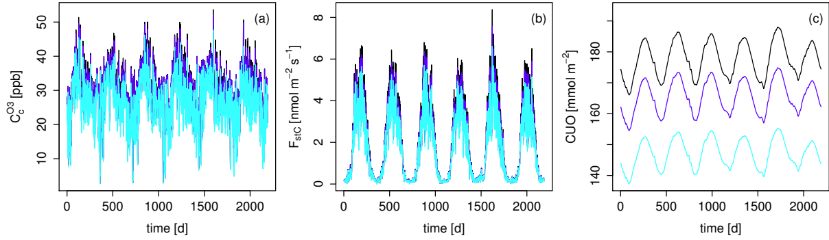
Figure 8. Mean daily values of the a) O_3 surface concentration [ppb], b) canopy integrated O_3 uptake into the leaves [ \text{nmol m}^{-2} \text{s}^{-1} ], and c) canopy integrated cumulative uptake of O_3 (CUO) [ \text{mmol m}^{-2} ] at the FLUXNET site FI-Hyy. Black: ATM model, Dark blue: D-STO model, Light blue: standard deposition model (D).
