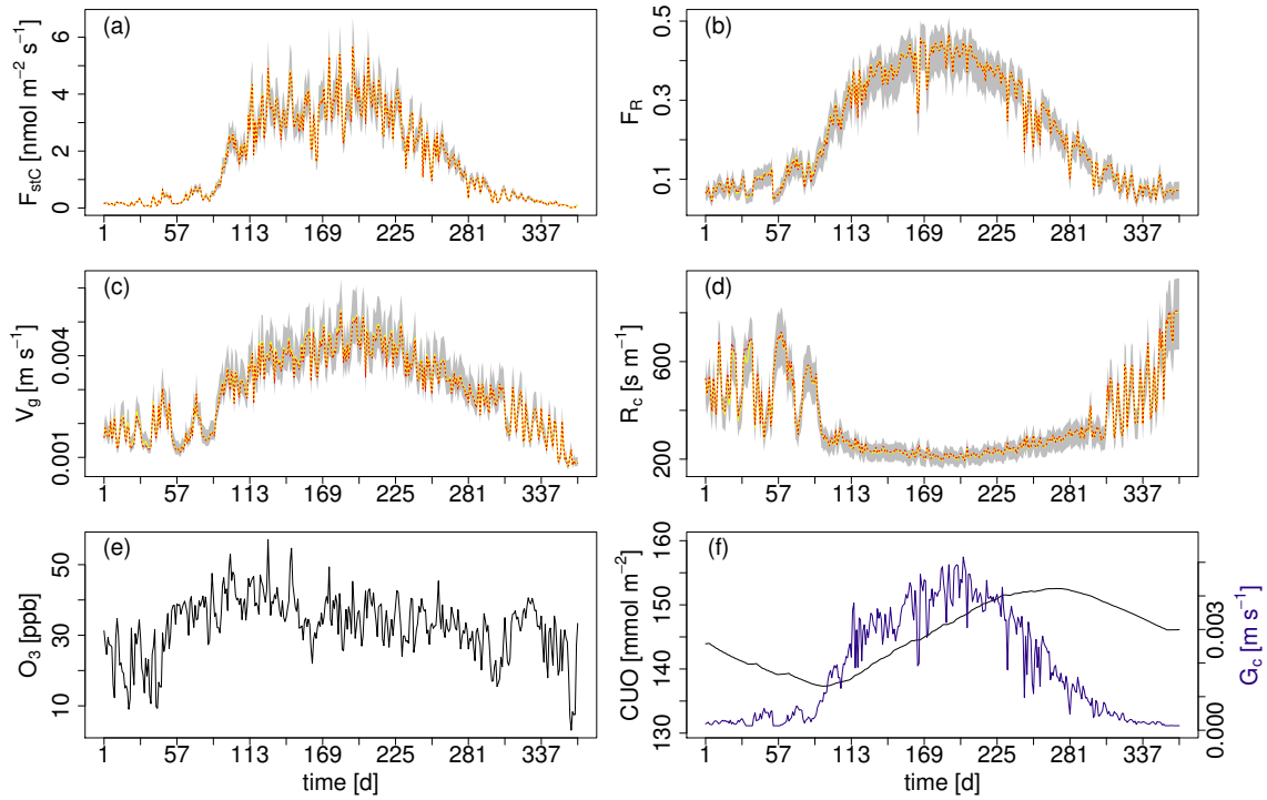
Figure 4. Ensemble range of key \text{O}_3 uptake/deposition variables resulting from the perturbation of R_a , b , r_{ext} , \hat{R}_{gs} and G_c within \pm 20\% of their central estimate. Shown are simulated daily mean values of a) \text{O}_3 uptake ( F_{stC} ), b) the \text{O}_3 flux ratio ( F_R ), c) \text{O}_3 deposition velocity ( v_g ) and d) \text{O}_3 surface resistance ( R_c ) for the boreal needle-leaved evergreen forest at the finish FLUXNET site FI-Hyy for the year 2001. Red dashed: unperturbed model; yellow: median of all sensitivity runs; light grey area: min-max-range off all sensitivity runs. Simulated daily mean values for the respective site and year of e) atmospheric \text{O}_3 concentrations \text{O}_3 and f) cumulative uptake of \text{O}_3 (CUO) and canopy conductance G_c .
