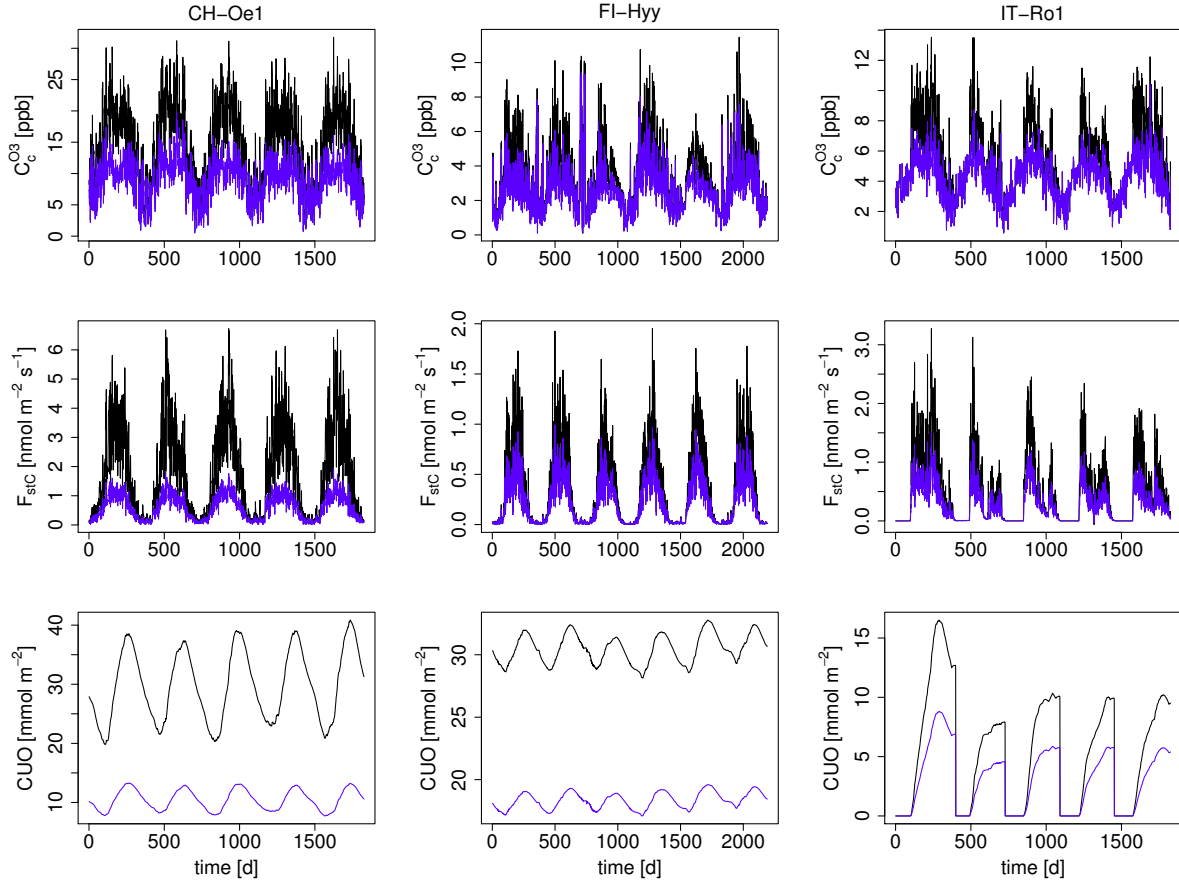
Figure 12. Differences in mean daily values of the a) \text{O}_3 surface concentration [ppb], b) canopy integrated \text{O}_3 uptake into the leafs [ \text{nmol m}^{-2} \text{s}^{-1} ], and c) canopy integrated cumulative uptake of \text{O}_3 (CUO) [ \text{mmol m}^{-2} ] for the three FLUXNET sites CH-Oe1, FI-Hyy and IT-Ro1. Blue: Difference between the D-STO model and the standard model (D), Black: Difference between the ATM model and the standard model (D).
