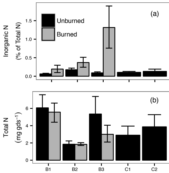
Figure 9. Bar chart showing the pulse of inorganic N relative to the total N pool size. Panel (a) shows the mean percent of inorganic N (i.e. NH 4 + and NO 3 - ) in soil under in unburned and burned periods. Panel (b) shows the mean total N soil content in burned and unburned periods, reported per gram of dry soil (gds). Error bars are ±95% CI.
