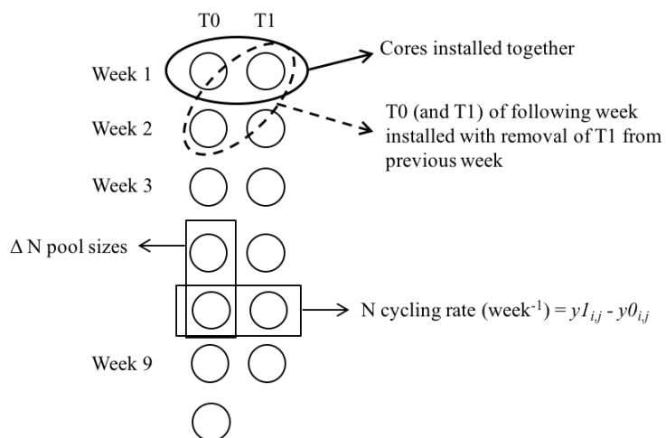
Figure 1. Schematic illustrating the paired-core sampling design across nine weeks throughout the growing season. Each circle represents the three soil cores and three incubated PVC collars installed every week.
