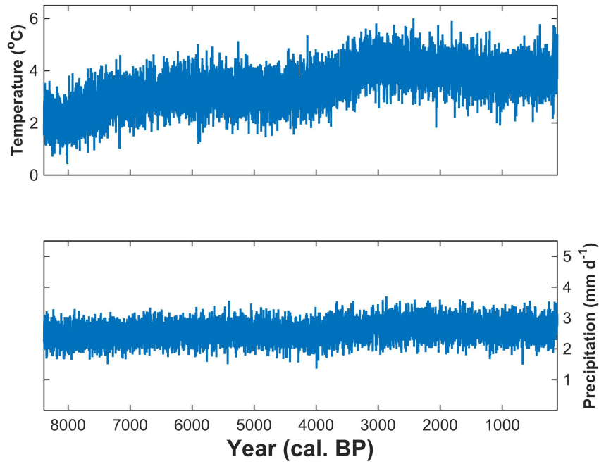
Fig. 4. Applied temperature ( ^{\circ}\text{C} ) and precipitation ( \text{mm}/\text{day} ) forcing for the last 8400 years at Mer Bleue
