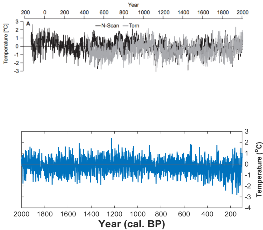
Fig. 5. Comparison between Esper et al. 2014 (Fig. 2a - N-Scandinavia/Finnish Lapland) and applied temperature ( ^{\circ}\text{C} ) forcing for the last 2000 years at Stordalen.
