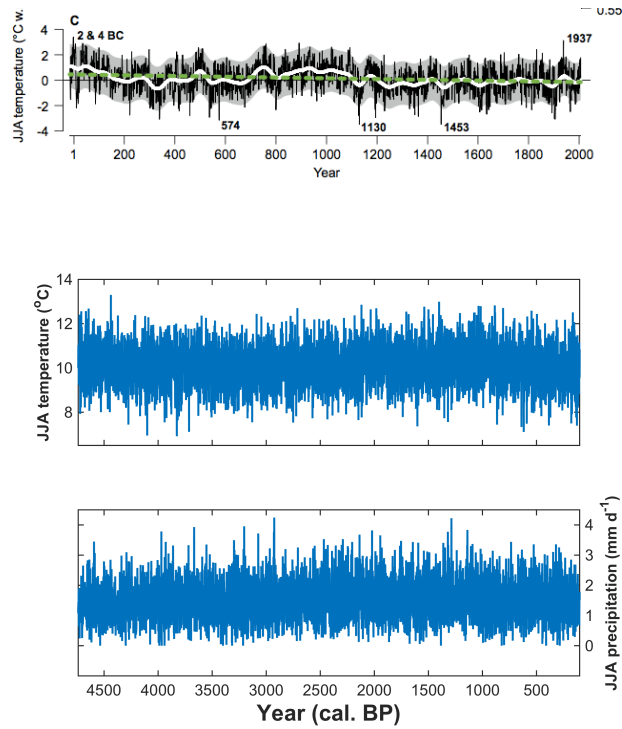
Fig. 6. Comparison between Esper et al. 2014 (Fig. 5c - northern Europe) and modelled June-July-August (JJA) temperature (°C) and precipitation (mm/day) at Stordalen
