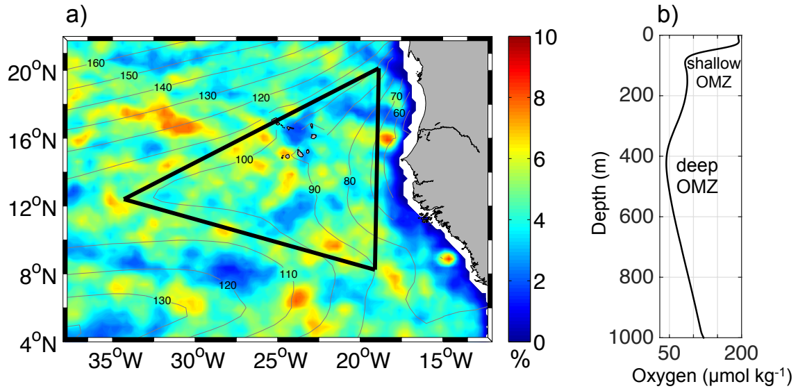
Figure 1: a) Map of the ETNA including contour lines of the oxygen minimum of the upper 200 m (in \mu\text{mol kg}^{-1} ) as obtained from the MIMOC climatology (Schmidtke et al., 2013). The color indicates the percentage of “dead-zone” eddy coverage per year. The black triangle defines the SOMZ. b) mean vertical oxygen profile of all profiles within the SOMZ showing the shallow oxygen minimum centered around 80 m depth and the deep oxygen minimum centered at 450 m depth.
