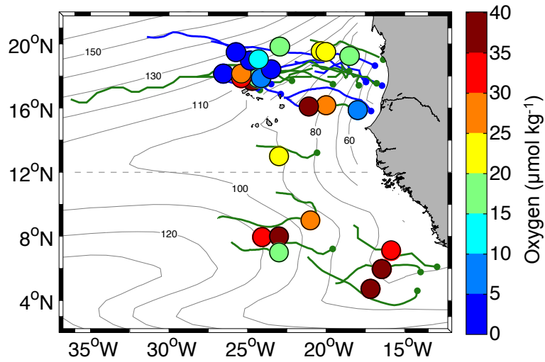
Figure 4: Minimum oxygen concentration (contour lines, \mu\text{mol kg}^{-1} ) in the ETNA between the surface and 200 m depth as obtained from the MIMOC climatology (Schmidtke et al., 2013). Superimposed colored dots are all low-oxygen measurements (below 40 \mu\text{mol kg}^{-1} in the upper 200 m) which could be associated with eddy-like structures. The size of the dots represents a typical size of the mesoscale eddies. The associated trajectories of the eddies are shown in green for ACMEs and in blue for cyclones. The oxygen concentrations are from the combined dataset of shipboard, mooring, glider and Argo float measurements.
