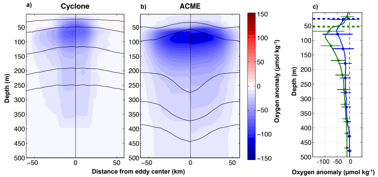
Figure 8: Vertical structure of oxygen from the composite a) CE and b) ACME in the ETNA presented as a half section across the eddies. The left side of both panels (-60 to 0 km) is based on reconstructed and measured oxygen profiles whereas the right side (0 to 60 km) is based on measured oxygen profiles only. Both methods are shown against the normalized radial distance. The grey lines represents the density surfaces inside the eddies. c) Mean profiles of the oxygen anomalies based on measured profiles only; green colors are associated to ACMEs and blue to CEs. Horizontal lines indicate the standard deviation of the oxygen anomaly at selected depths. The thick dashed lines indicates the mean ML within the different eddy types. The grey vertical dashed line represents zero oxygen.
