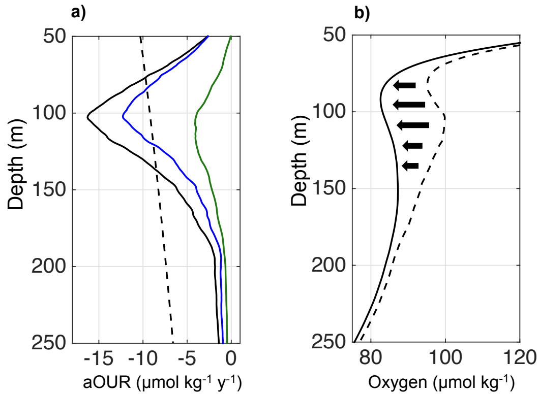
Figure 9: a) Depth profile of the apparent oxygen utilization rate (aOUR, \mu\text{mol kg}^{-1} \text{y}^{-1} ) for the Atlantic as published from Karstensen et al. (2008) (dashed black line). The oxygen consumption profile due to low-oxygen eddies referenced for the SOMZ region (solid black line) and the separation into CEs (blue) and ACMEs (green). The solid black line in b) represents the observed mean vertical oxygen profile of all profiles within the SOMZ against depth, whereas the dashed black line represents the theoretical vertical oxygen profile in the SOMZ without the dispersion of low-oxygen eddies. Naturally due to the dispersion of negative oxygen anomalies, the observed values (black line) are lower than the theoretical oxygen concentrations in the SOMZ without eddies (dashed black line). The impact of the dispersion of low-oxygen eddies on the oxygen budget in the depth of the shallow oxygen minimum zone are also indicated by the thick black arrows.
