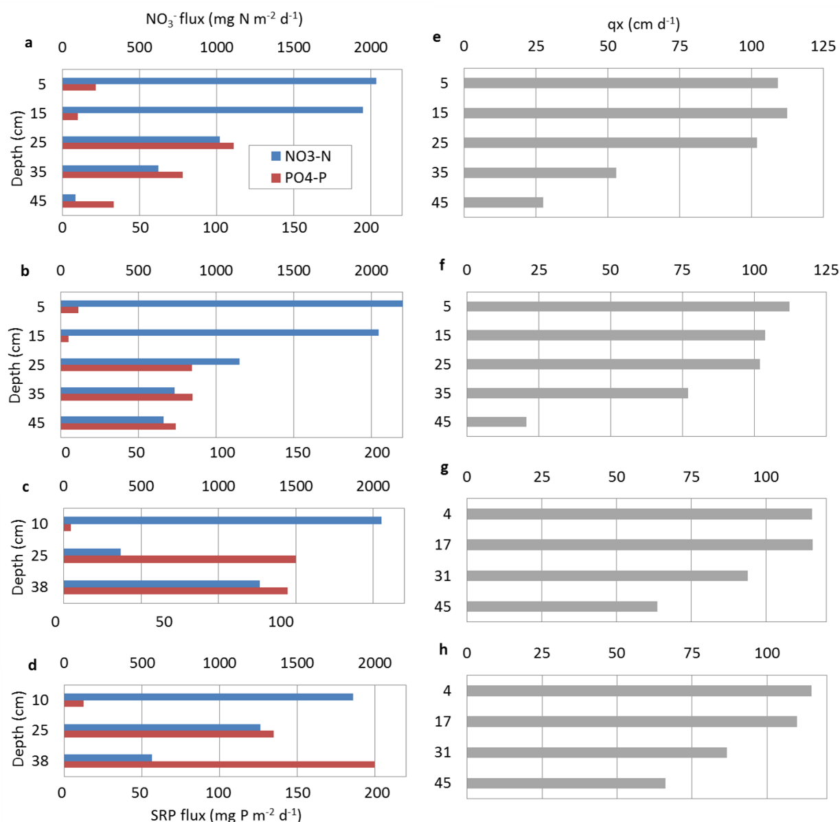
Figure 3. Time integrative measurements for the 04.-11.06.2015. Left side: Horizontal NO 3 - -N and SRP-P flux in mg m -2 d -1 through the resin HPFM R1 (a), R2 (b) and the layered HPFM L5 (c) and L6 (d). Right side: corresponding Darcy velocities q_x in cm d -1 through the activated carbon HPFM AC3 (e) and AC4 (f) and the layered HPFMs 5L (g) and 6L (h)
