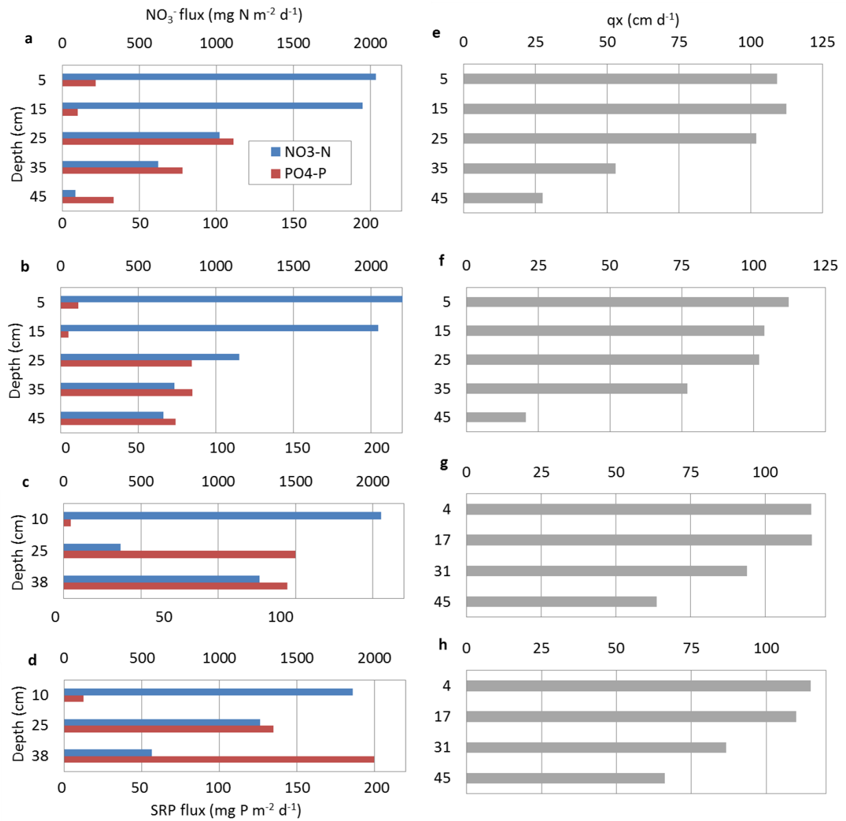
Figure 3. Time integrative measurements for the 04.-11.06.2015. Left side: Horizontal NO 3 - -N and SRP-P flux in mg m -2 d -1 through the resin HPFM R1 (a), R2 (b) and the layered HPFM L5 (c) and L6 (d). Right side: corresponding Darcy velocities q_x in cm d -1 through the activated carbon HPFM AC3 (e) and AC4 (f) and the layered HPFMs 5L (g) and 6L (h)
