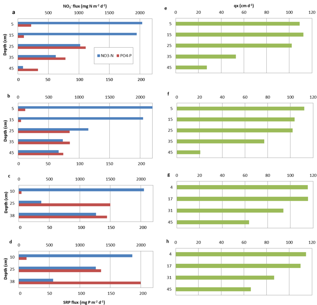
Figure 3. Time integrative measurements for the 04.-11.06.2015. Left side: Horizontal \text{NO}_3^- -N and SRP-P flux in \text{mg m}^{-2} \text{d}^{-1} through the resin HPFMs R1 (a), R2 (b) and the layered HPFMs L5 (c) and L6 (d). Right side: corresponding Darcy velocities q_x in \text{cm d}^{-1} through the activated carbon HPFMs AC3 (e) and AC4 (f) and the layered HPFMs 5L (g) and 6L (h).
