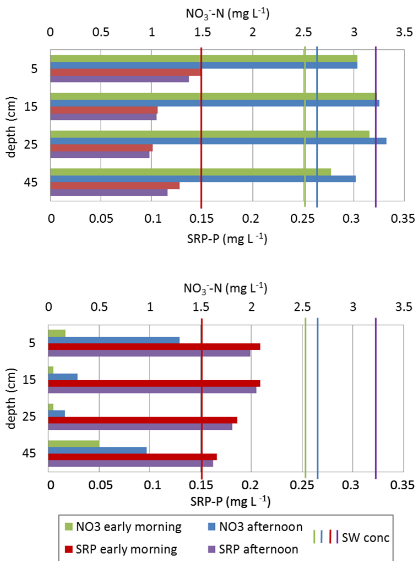
Figure 6. Concentrations of NO 3 - -N and SRP in time differentiating manually taken pore-water samples from MLS A (bottom) and MLS B (top) on 8 th October 2015. Corresponding surface water concentrations are marked as vertical lines.
