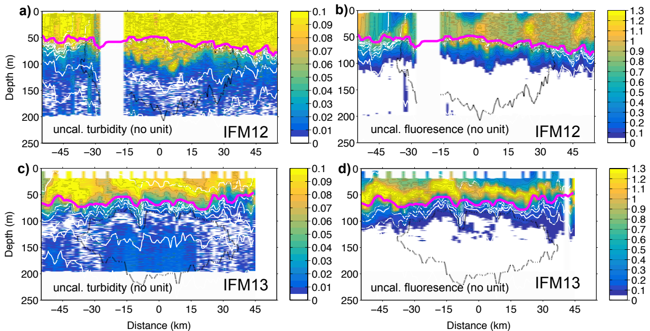
Figure 6: Uncalibrated turbidity (a, c) and chlorophyll-fluorescence (b,d) data from glider IFM12 survey (a, b) and glider IFM13 survey (c, d). The magenta line denoted the base of the mixed layer, the broken black line is the extend of the low oxygen core ( \text{oxygen} < 40 \mu\text{mol kg}^{-1} ).
