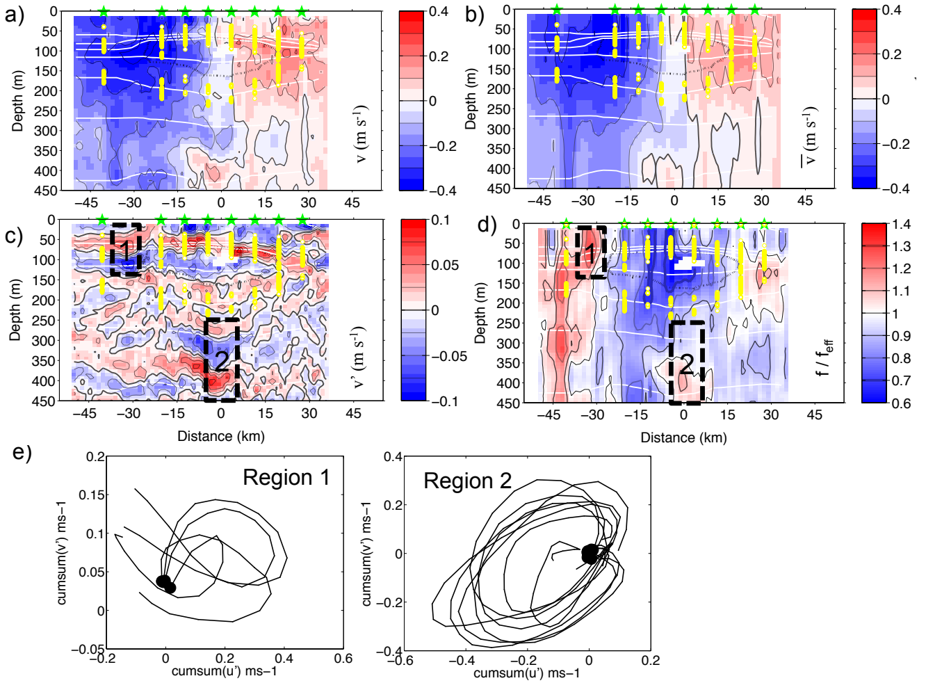
Figure 5: a) observed meridional velocity, b) boxcar filtered meridional velocity (applied over 150 m), c) difference between observed and boxcar filtered velocity. The thick black broken line indicates the 40 \mu\text{mol kg}^{-1} oxygen concentration, white contours are selected density anomaly contours ( \Delta\sigma=0.2 \text{ kg m}^{-3} ) determined by gridding CTD profile data (see green stars at 0 dbar for station positions). The yellow dots indicate the N^2 maximum from CTD profile data. d) Ratio between local Coriolis parameter ( f ) and the effective Coriolis parameter ( f_{\text{eff}} ). e) Progressive vector diagram of v' for region 1 (250 to 450m depth) and 2 (20 to 140 m) (see c) and d) for locations), black dots marks the shallowest depth
