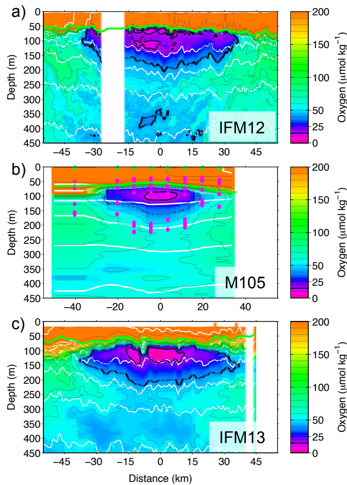
Figure 2: Oxygen distribution from the three eddy surveys (see Figure 1) in reference to distance (0 km is set at a subjectively selected eddy centre): a) Glider IFM12, b) ship M105, and c) glider IFM13. The 15 \mu\text{mol kg}^{-1} ( 40 \mu\text{mol kg}^{-1} ) oxygen contour is indicated as a bold (broken) black line, selected density anomaly contours are shown as white lines ( \Delta\sigma = 0.2 \text{ kg m}^{-3} ). The green line indicates the mixed layer base. The oxygen contour in b) was gridded based on the 8 CTD stations (locations indicated by green stars at 0dbar) and mapped to a linear section in latitude, longitude. In b) the magenta dots indicate positions of local N^2 maxima in the CTD profiles.
