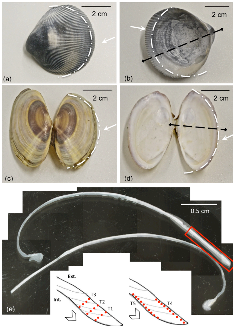
5 Figure 2: Photographs of external (left) and internal (right) views of bivalves. Fulvia tenuicostata (a,b); Soletellina biradiata (c, d). (e) Photo-mosaic showing ventral margin ( S. biradiata ) as seen in thin section. Powder was sampled from the ventral margin for x-ray diffraction analysis (white dashed lines and arrows: a, b, c and d). The area adjacent to the ventral margin was then targeted for confocal Raman microscopy, LA-ICP-MS and EPMA (red box: e). Lower panel show representation of laser spots along five transects (T1–T5). T1–T3 are parallel to the shell edge and T4 and T5 are parallel to the external and internal shell margin (respectively).
