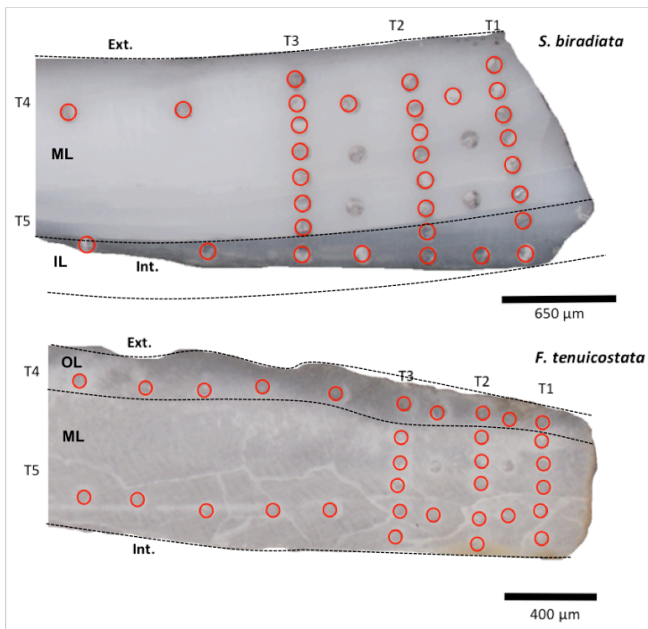
5 Figure 9: Location of laser spots along five transects. T1–T3 transects towards the inner shell surface and parallel to each other. T4 along the outer portion of the outer shell layer and T5 along the inner portion of the outer shell layer. Inner and outer portion of the outer shell layer indicates by Int. and Ext. respectively. Shell layers indicated by OL: outer layer and ML: middle layer, and IL: internal layer. Note: absence of outer shell layer and inner shell layer in these sections of S. biradiata and F. tenuicostata respectively. T4 and T5 were sampled from different shell layers as labelled.
