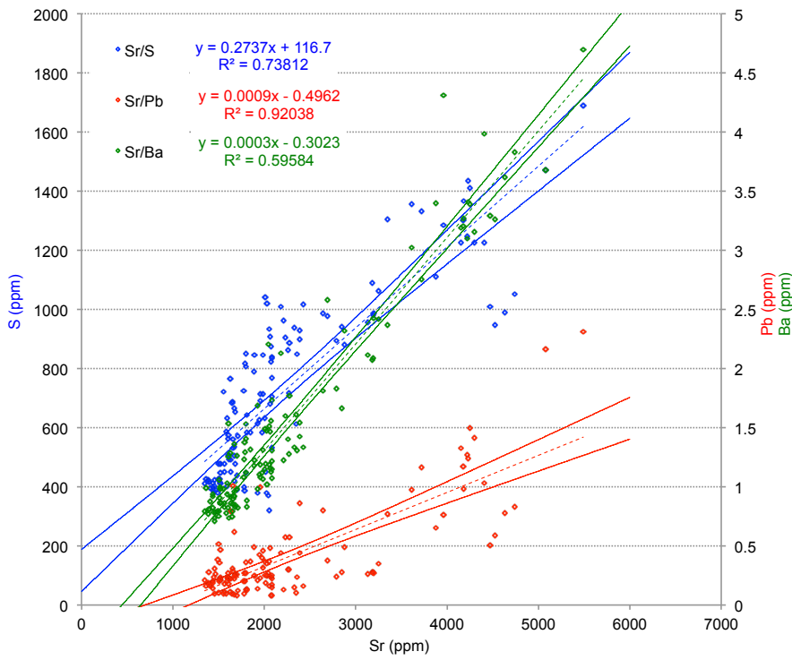
Figure 12: Graphs showing significant linear correlations and 95% confidence intervals of LA-ICP-MS measurements for F. tenuicostata (Mg/P, Mg/S and Sr/P) and S. biradiata (Sr/S, Sr/Pb and Sr/Ba)
