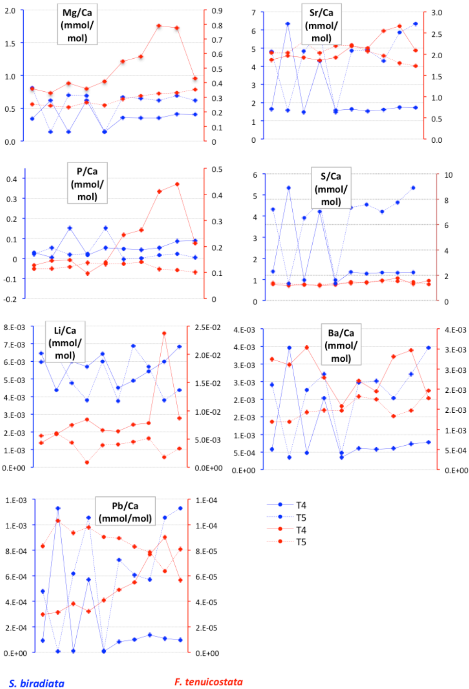
Figure 11: LA-ICP-MS results for T4 and T5 transects. Blue lines represent results for S. biradiata (G171) and red lines represent results for F. tenuicostata (G155). For visual clarity the uncertainty estimates are not presented on the graphics but are as follow: S. biradiata Li 1\sigma = 0.03 , Mg 1\sigma = 0.26 , P 1\sigma = 0.18 , S 1\sigma = 2.2 , Sr 1\sigma = 1.7 , Ba 1\sigma = 0.001 , Pb 1\sigma = 2.24E-4 , and F. tenuicostata Li 1\sigma = 0.05 , Mg 1\sigma = 0.24 , P 1\sigma = 0.3 , S 1\sigma = 1.78 , Sr 1\sigma = 1.0 , Ba 1\sigma = 0.001 , Pb 1\sigma = 1.0E-04 .
