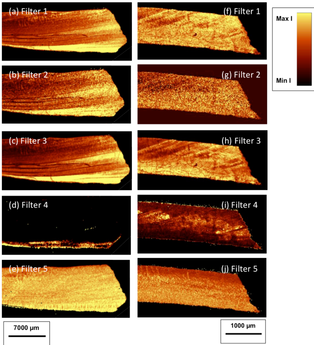
5 Figure 6: Images extracted from filters applied to the Raman spectra (see Fig. 5) from samples G171 ( S. biradiata ) (a-e), and G155 ( F. tenuicostata ) (f-j). Scale bar: 7000 μm (a-e), 1000 μm (f-j). Colour scale: bright colours correspond to high intensities (high CCD counts) and dark colours correspond to low intensities (low CCD counts). Sub-horizontal and curved lines, most visible in (a)-(c) and (f)-(h), are structural features of the shells. Scale bar: 500 μm.
