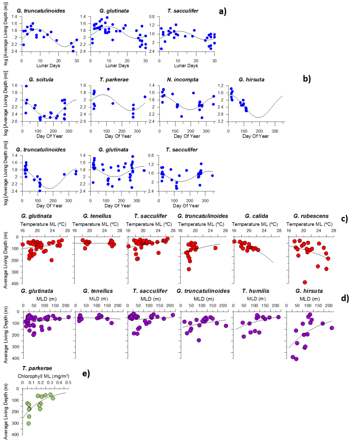
Figure 9. Comparison of modelled and observed ALD in species where ALD appears to be predictable (p-value < 0.05, Table 3) by (a) lunar cycle, (b) yearly cycle, (c) mean temperature in the mixed layer interval, (d) mixed layer depth and (e) mean chlorophyll a concentration in the mixed layer interval.
