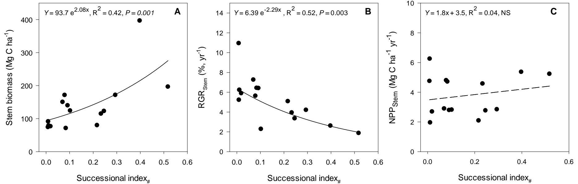
Figure S4S2. Biomass (a) , relative growth rates (RGR b ) and net primary production (NPP c ) of stems including branches of each plot in relation to its successional index, based on number of stems (#) of the most abundant early and late successional species (eq 9). Biomass, RGR, and NPP is calculated from eq. 3, 6, 5, respectively based on measurements of D_{BH} , H and \rho . The adjusted R^2 -values are 0.37 and 0.48 in a and b, respectively.
