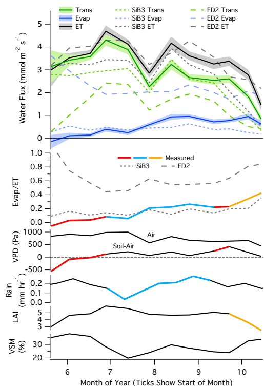
5 Figure 4: Composite seasonal cycles (including the years 2012 and 2013) of daytime evapotranspiration (ET), transpiration, and evaporation, as estimated here and as predicted by the ED2 and SiB3 models, along with: the ratio of evaporation (Evap) to ET, the atmospheric vapor pressure deficit (VPD), the soil-atmosphere vapor pressure difference, rainfall, the leaf area index (LAI), and the volumetric soil moisture content between 0 and 30 cm depth (VSM). Lines connect the mean values of each 2-week bin. Pale bands depict standard errors in the means as estimated from the variability within each bin. The soil-air vapor pressure difference is based on the assumption of saturated air at the soil surface and therefore reflects the maximum possible difference. Color-coding in the lower panels highlights which environmental control is dominating the behavior of the Evap/ET ratio. Model output was filtered to include only times when measurements were made.
