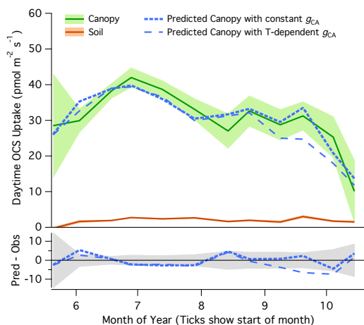
Figure 2: Composite seasonal cycles (including the years 2012 and 2013) of daytime soil uptake, canopy uptake, and predicted canopy uptake from Eq. (1), along with the differences between predicted and observed canopy uptake. Lines connect the mean values of each 2-week bin. Pale bands depict standard errors in the means as estimated from the variability within each bin.
