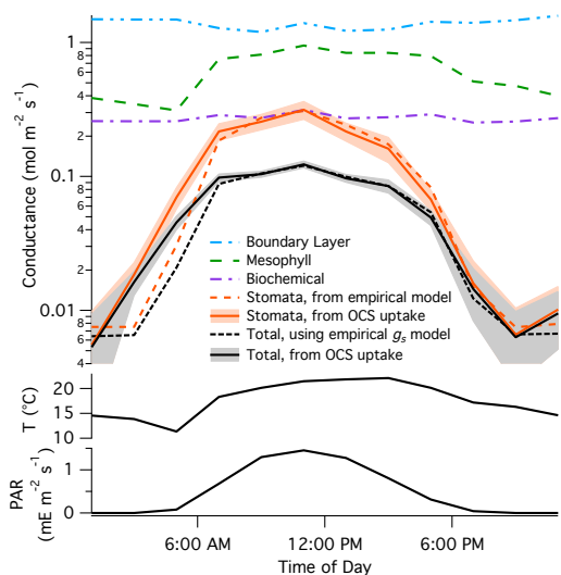
Figure 3: Composite diel cycles (including May through October of 2012 and 2013) of the expected leaf boundary layer, stomatal, mesophyll, biochemical, and total conductances to OCS transport and chemical destruction, along with the stomatal and total conductances derived from OCS uptake. Lower panels show air temperature and PAR for context. Lines connect the mean values of each 2-hour bin. Pale bands depict standard errors in the means as estimated from the variability within each bin. The boundary layer conductance is likely overestimated at night (see text).
