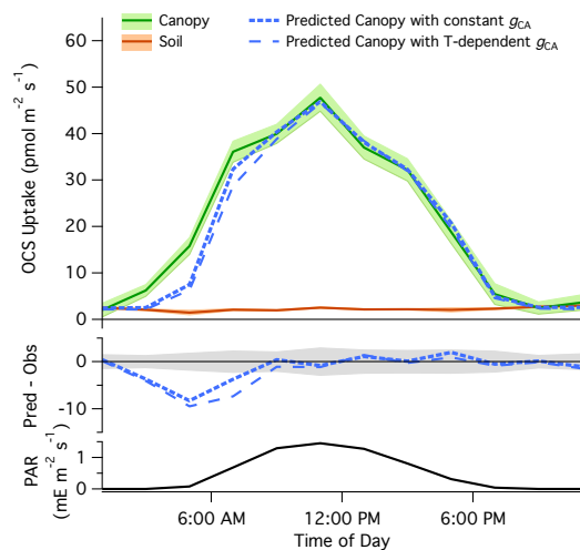
Figure 1: Composite diel cycles (including May through October of 2012 and 2013) of soil uptake, canopy uptake, and predicted canopy uptake from Eq. (1), along with the differences between predicted and observed canopy uptake, and photosynthetically active radiation (PAR) for reference. Lines connect the mean values of each 2-hour bin. Pale bands depict standard errors in the means as estimated from the variability within each bin.
