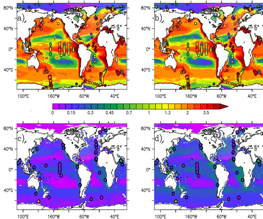
Figure 6. Sequestration of POC. The panels on the left show POC fluxes for the simulation without the lability parameterisation, i.e. \text{POC}_{\text{sPOC}} and \text{GOC}_{\text{bPOC}} have a single lability (noRC). Those on the right are with the lability parameterisation (RC). The upper two panels (a, b) show the modelled flux at 100 m; the observations are from the same depth \pm 20 m. Panels (c) and (d) show the flux through 2000 m; the observations are at the same depth \pm 400 m. The datasets used in these figures are from Dunne et al. (2005), Gehlen et al. (2006) and Le Moigne (2013). Fluxes are in \text{mol m}^{-2} \text{yr}^{-1} .
