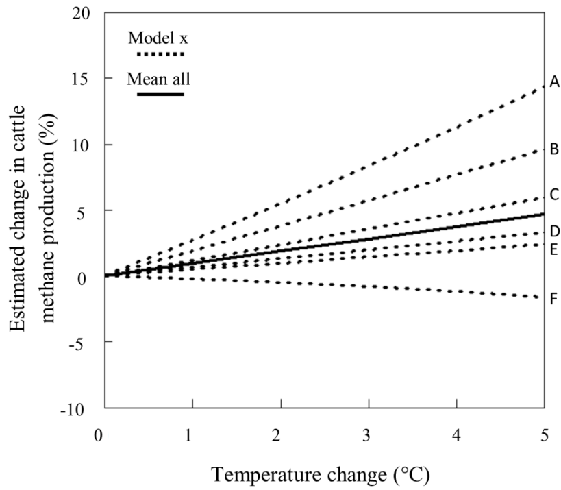
730 Figure 3: Estimated change in cattle methane production with temperature derived declines in grass nutritive quality. Dotted lines represent six model outputs as defined by equations A – F (defining relationships between grass nutritive quality and methane production) when combined with the inverse relationship between temperature and grass nutritive quality presented in this article. The continuous line represents the mean weighted model; mean methane production predicted by all six equations, weighted by the number of contributing datasets.
