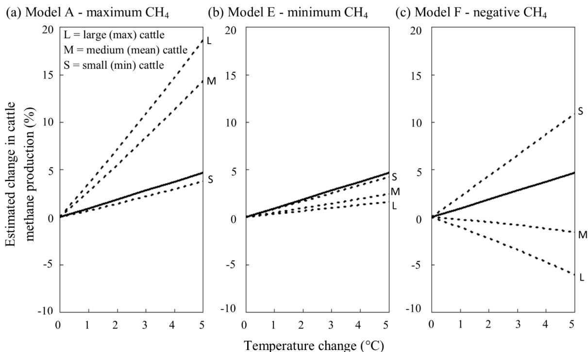
Figure 4: Estimated change in enteric methane production with temperature change for (a) the model predicting the largest increases in methane production (maximum CH 4 ), (b) the model predicting the lowest increase in methane production (minimum CH 4 ) and (c) the model which predicts both increases and decreases in methane production (negative CH 4 ).
