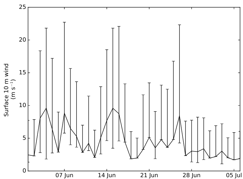
Figure 8. Time series of daily mean surface 10 10-m wind speed [ \text{m s}^{-1} ] observed at the Resolute airport ( located within 7 km of the study site ) during the melt period in 2010. The upper and lower vertical bars associated with the daily mean values represent the daily maximum and minimum values, respectively.
