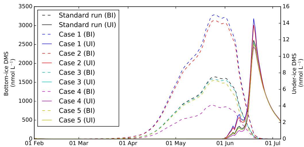
Figure 7. Simulated time series of bottom-ice (BI) and under-ice (UI; 0.5 m below the ice) DMS concentrations [nmol L -1 ] during 2010 for: the standard run; Case 1: doubling the intracellular DMSP:Chl a ratio; Case 2: doubling the DMS yield fraction; Case 3: doubling the bacterial DMSPd consumption rate constant; Case 4: doubling the bacterial DMS consumption rate constant; and Case 5: doubling the photolysis rate constant.
