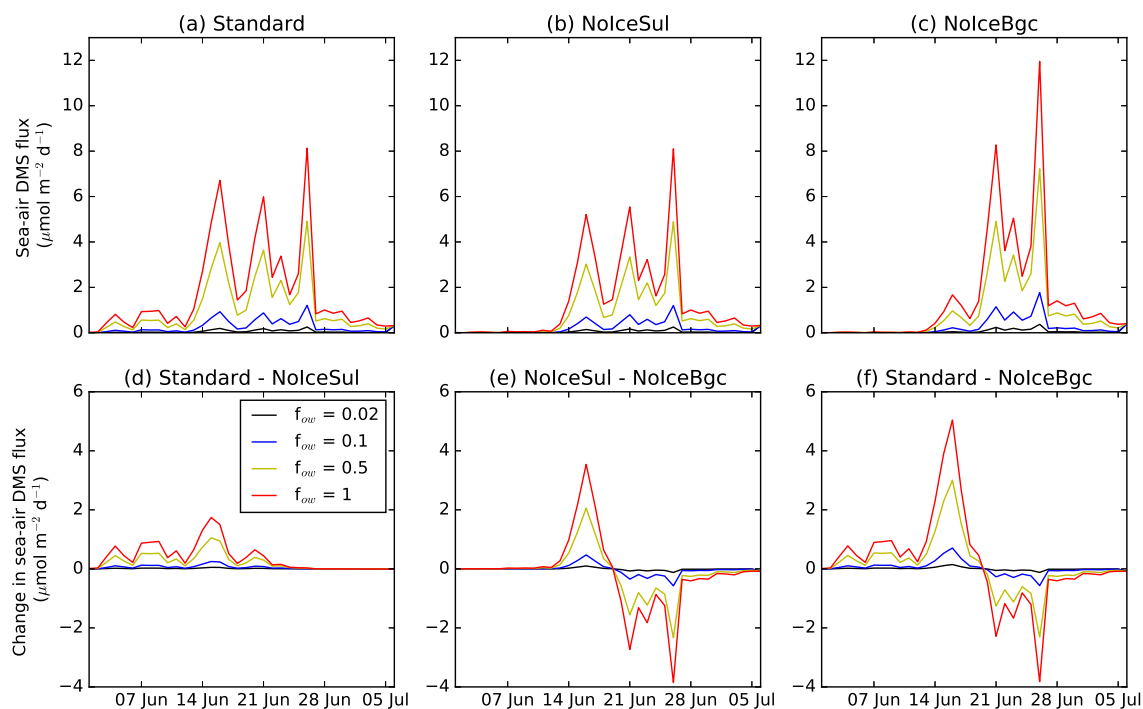
Figure 9. Simulated time series of sea-air DMS fluxes [ \mu\text{mol m}^{-2} \text{d}^{-1} ] for (a) the standard run and the sensitivity runs that excluded (b) the sea-ice sulfur cycle (NoIceSul) and (c) both the sea-ice sulfur cycle and ecosystem (NoIceBgc) and the flux difference between (d) the standard and NoIceSul runs, (e) the NoIceSul and NoIceBgc runs, and (f) the standard and NoIceBgc runs during the melt period in 2010. In (d), (e), and (f), positive values represent enhancement in the simulated flux due to the incorporation of sea-ice sulfur cycle, ecosystem, and both sulfur cycle and ecosystem, respectively, while negative values represent reduction.
