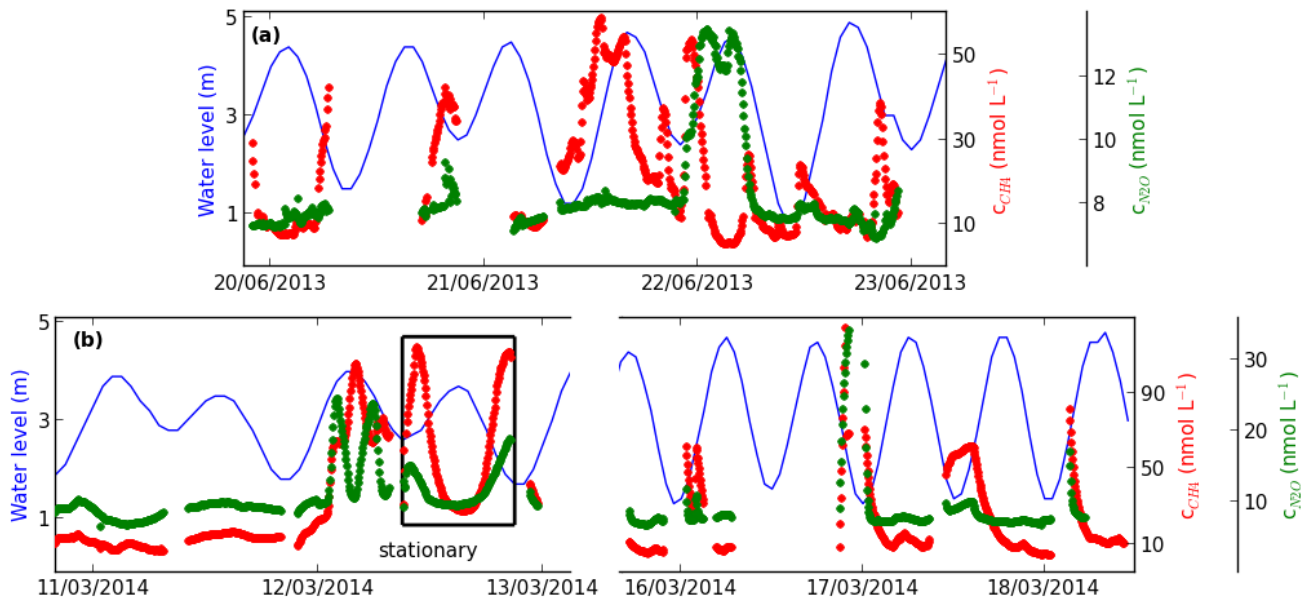
Figure 4: Time series of methane and nitrous oxide concentrations in the Lupar and Saribas estuaries measured during the dry season (2013) campaign (upper panel) and the wet season campaign (lower panel) and the water level as predicted for Pulau Lakei (+1 h for Lupar and Saribas). Spatial, temporal and tidal variations are overlapping in the Figure. One stationary measurement, as recorded on the Saribas River in 2014, is denoted with the black box. Note the discontinuous time axis in the lower panel.
