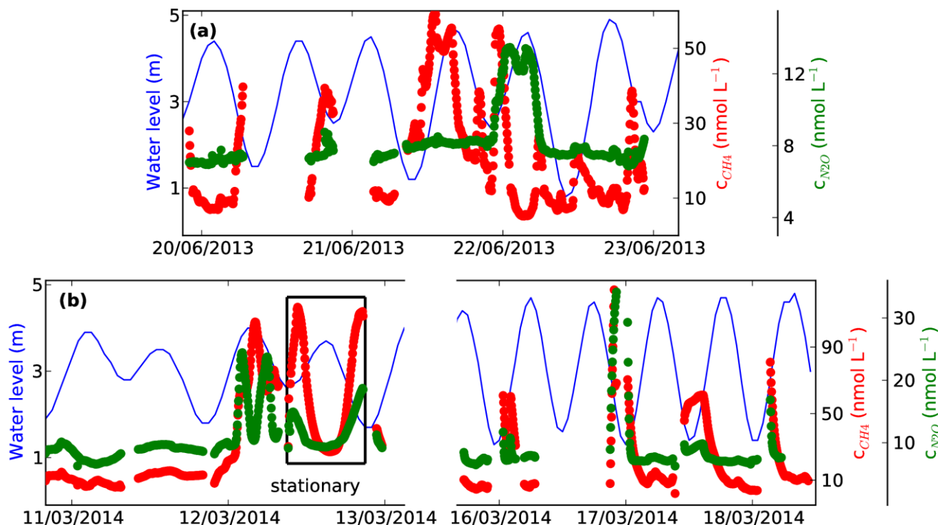
Figure 4: Time series of methane and nitrous oxide concentrations in the Lupar and Saribas estuaries measured during the dry season (2013) campaign (upper panel) and the wet season campaign (lower panel) and the water level as predicted for Pulau Lakei (+1 h for Lupar and Saribas). Spatial, temporal and tidal variations are overlapping in the Figure. One stationary measurement, as recorded on the Saribas river in 2014, is denoted with the black box. Note the discontinuous time axis in the lower panel.
