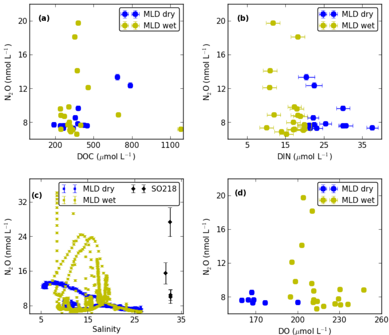
Figure 2: Relationship of nitrous oxide concentrations with (a) dissolved organic carbon (DOC), (b) dissolved inorganic nitrogen (DIN), (c) salinity and (d) dissolved oxygen (DO). MLD refers to the campaigns on the Lupar and Saribas estuaries in the dry and wet season, respectively, SO218 denotes data from the R/V Sonne cruise.
