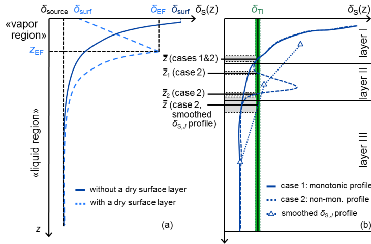
2 3 Figure 2: (a) Simulated soil water isotopic composition ( \delta_s ) profiles, for a water saturated (dark blue line) and 4 unsaturated (light blue dotted line) soil following Barnes and Allison (1983). Indices “surf” and “EF” refer to soil 5 surface and Evaporation Front. “vapor” and “liquid” regions refer to soil regions where water flow occurs 6 predominantly in the liquid and vapor phase, respectively. (b) Illustration of the “graphical inference” method for 7 determining the “mean root water uptake depth” ( \bar{z} ). “Ti” stands for the sap xylem water at the plant tiller. Case 1: 8 one unique solution is found; case 2: more than one solution is found. Smoothed profile is designated by the symbols). 9 \bar{z} range is indicated by the gray horizontal stripes.
