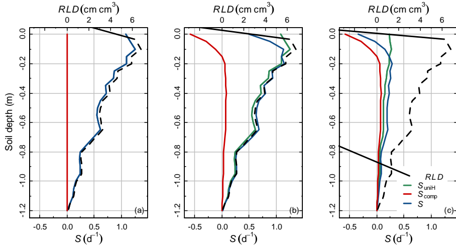
3 4 Figure 1: Some examples of root water uptake sink term ( S , in d^{-1} ) profiles (blue lines) conceptualized as the sum of 5 S_{uniH} (green lines), the root water uptake term proportional to root length density RLD (dotted black line) and the 6 compensatory root water uptake ( S_{comp} , red lines). (a) S_{comp} = 0 (no root compensation) leading to S = S_{uniH} . (b) S_{comp} \neq 7 0 and becomes negative towards the surface but remains smaller (in absolute term) than S_{uniH} . (c) S_{comp} \neq 0 and is 8 negative at the surface while is greater than S_{uniH} for z > -0.08 m. In the last case, S is negative at the surface, meaning 9 hydraulic lift is observed.
