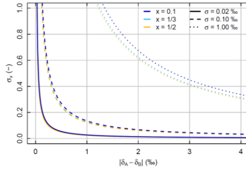
2 3 Figure 3: Standard error ( \sigma_x ) associated with the estimation of the relative contribution ( x ) of source A water to root 4 water uptake in case of two distinct sources (A and B of isotopic compositions \delta_A and \delta_B ). Three x values (0.1, dark 5 blue color; 1/3, light blue; 1/2, orange) and three values of standard errors associated with sampling and measurement 6 of \delta_A , \delta_B , and of the isotopic composition of the tiller sap water ( \delta_T ) (0.02, solid line; 0.10, and 1.00, dashed lines) are 7 tested.
