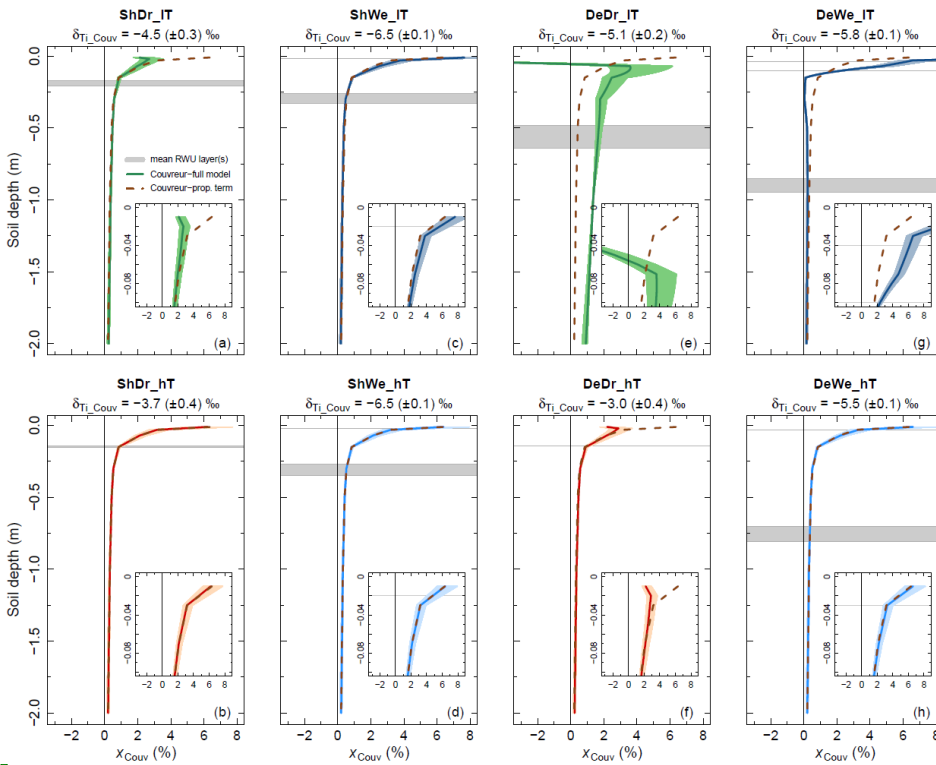
2 3 Figure 4: Simulated depth ( z , in m) profiles of x_{Couv} (%) (solid colored lines), the simulated relative contributions to 4 transpiration provided by the model of Couvreur et al. (2012), for experiments “ShDr” (soil with shallow groundwater 5 table and relatively dry soil surface), “ShWe” (soil with shallow groundwater table after a rainfall event), “DeDr” 6 (soil with deep groundwater table with relatively dry soil surface), “DeWe” (soil with deep groundwater table and wet 7 soil surface ). Suffices “IT” and “hT” refer to “low” and “high” transpiration rate simulations. The color-shaded areas 8 depict the uncertainty of the model estimates on the account of the precision of the measurements. The horizontal 9 gray-shaded areas delimit the mean root water uptake layer(s) obtained by the “graphical inference” method . At the 10 bottom right corner of each plot is a detail presented for z \geq -0.10 m. Finally, results from the first term of the model 11 of Couvreur et al. (2012) which considers uptake proportional to root length density is plotted as a dashed brown line 12 for comparison. Note that negative x_{Couv} means hydraulic redistribution by the roots.
