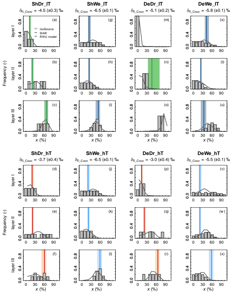
Figure 6: Simulated ranges of possible relative contributions to transpiration from three defined soil layers (I: 0.00 – 0.05 m, II: 0.050 – 0.225 m, and III: 0.225 – 2.000) provided by the multi-source mixing model IsoSource (Phillips and Gregg, 2003) (displayed in the form of gray histograms). Density distribution functions following the Bayesian model SIAR (Parnell et al., 2010) (gray lines). “Sh” (“De”) stands for the virtual experiments where the soil has a shallow (deep) groundwater table while “Dr” and “We” stand for when the soil is dry or wet at the surface. Suffices “IT” and “hT” refer to “low” and “high” transpiration rate simulations. The colored vertical lines give x_{I,Couvr} , x_{II,Couvr} , and x_{III,Couvr} , the relative contributions to transpiration from layers I, II, and III simulated by the analytical model of Couvreur et al. (2012). The color-shaded areas associated with x_{I,Couvr} , x_{II,Couvr} , and x_{III,Couvr} refer to their uncertainty associated with input data uncertainty.
