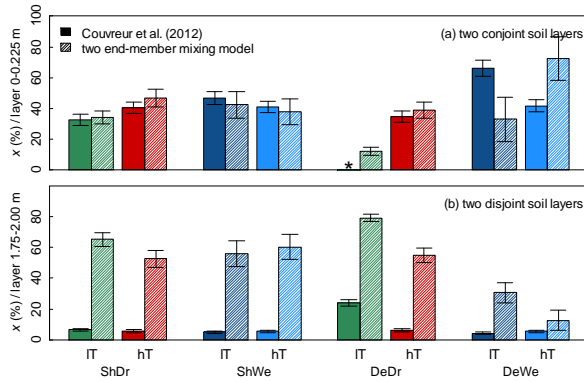
Figure 5: Comparison between relative contributions to transpiration ( x , in %) simulated by the analytical RWU model of Couvreur et al. (2012) and the two end-member mixing model in case of two defined soil layers. Figure 5a displays x from the topmost soil layer (0 - 0.225 m) in case of a two conjoint soil layers (0 - 0.225 m and 0.225 - 2.00 m) whereas Figure 5b displays x from the lowest soil layer (1.75 - 2.00 m) in case of a two disjoint soil layers (0 - 0.225 m and 0.225 - 2.00 m), i.e., information on soil water isotopic composition is lacking between 0.225 and 1.75 m. “Sh” (“De”) stands for the virtual experiments where the soil has a shallow (deep) groundwater table while “Dr” and “We” stand for when the soil is dry or wet at the surface. Suffices “IT” and “hT” refer to “low” and “high” transpiration rate simulations. “*” refers to when hydraulic redistribution is simulated by the analytical model, leading to a negative x . Error bars are either one standard deviation (for the RWU analytical model) or one standard error (for the TM approach).
