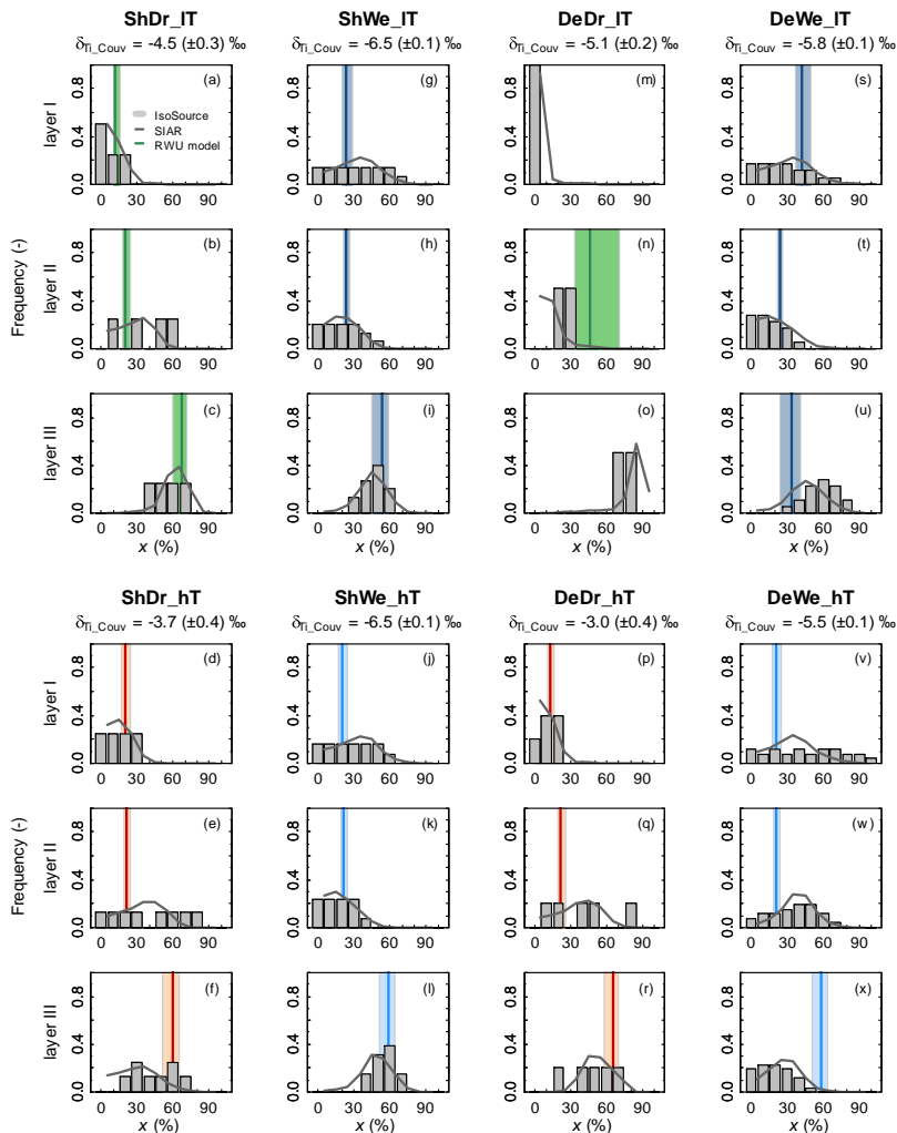
Figure 7: Simulated ranges of possible relative contributions to transpiration from three defined soil layers (I: 0.00 – 0.05 m, II: 0.050 – 0.225 m, and III: 0.225 – 2.000) provided by the multi-source mixing model IsoSource (Phillips and Gregg, 2003) (displayed in the form of gray histograms). Density distribution functions following the Bayesian model SIAR (Parnell et al., 2010) (gray lines). “Sh” (“De”) stands for the virtual experiments where the soil has a shallow (deep) groundwater table while “Dr” and “We” stand for when the soil is dry or wet at the surface. Suffices “IT” and “hT” refer to “low” and “high” transpiration rate simulations. The colored vertical lines give x_{I\_Couv} , x_{II\_Couv} , and x_{III\_Couv} , the relative contributions to transpiration from layers I, II, and III simulated by the analytical model of Couvreur et al. (2012). The color-shaded areas associated with x_{I\_Couv} , x_{II\_Couv} , and x_{III\_Couv} refer to their uncertainty associated with input data uncertainty.
