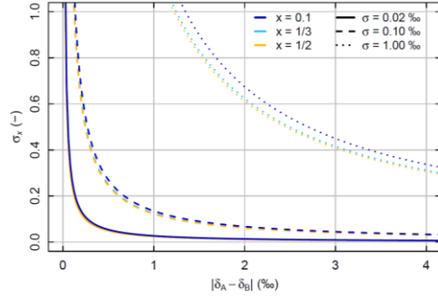
2 3 Figure 4: Standard error ( \sigma_x ) associated with the estimation of the relative contribution ( x ) of source A water to root 4 water uptake in case of two distinct sources (A and B of isotopic compositions \delta_A and \delta_B ). Three x values (0.1, dark 5 blue color; 1/3, light blue; 1/2, orange) and three values of standard errors associated with sampling and measurement 6 of \delta_A , \delta_B , and of the isotopic composition of the tiller sap water ( \delta_{TI} ) (0.02, solid line; 0.10 and 1.00, dashed lines) are 7 tested.
