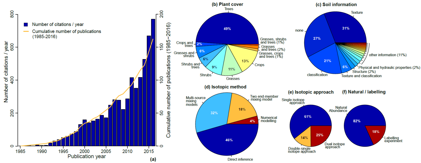
2 3 Figure 3: Evolution of the number of citations per year and cumulative number of publications from 1985 to 2016 (a). Details are given on the plant cover (b), the available soil 4 information (c), the applied isotopic method (d) and approach (e), and the type of experiment (f).
