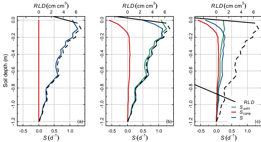
Figure 1: Some examples of root water uptake sink term ( S , in d^{-1} ) profiles (blue lines) conceptualized as the sum of S_{uniH} (green lines), the root water uptake term proportional to root length density RLD (dotted black line) and the compensatory root water uptake ( S_{comp} , red lines). (a) S_{comp} = 0 (no root compensation) leading to S = S_{uniH} . (b) S_{comp} \neq 0 and becomes negative towards the surface but remains smaller (in absolute term) than S_{uniH} . (c) S_{comp} \neq 0 and is negative at the surface while is greater than S_{uniH} for z > -0.08 m. In the last case, S is negative at the surface, meaning hydraulic lift is observed.
