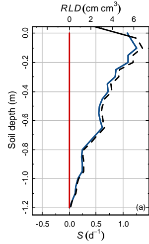
Deleted: Figure 1: Some examples of root water uptake sink term ( S , in d^{-1} ) profiles (blue lines) conceptualized as the sum of S_{uniIT} (green lines), the root water uptake term proportional to root length density RLD (dotted black line) and the compensatory root water uptake ( S_{comp} , red lines). (a) S_{comp} = 0 (no root compensation) leading to S = S_{uniIT} . (b) S_{comp} \neq 0 and becomes negative towards the surface but remains smaller (in absolute term) than S_{uniIT} . (c) S_{comp} \neq 0 and is negative at the surface while is greater than S_{uniIT} for z > -0.08 m. In the last case, S is negative at the surface, meaning hydraulic lift is observed.
