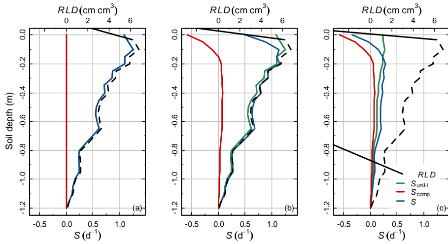
2 3 Figure 1: Some examples of root water uptake sink term ( S , in d^{-1} ) profiles (blue lines) conceptualized as the sum of 4 S_{uniH} (green lines), the root water uptake term proportional to root length density RLD (dotted black line) and the 5 compensatory root water uptake ( S_{comp} , red lines). (a) S_{comp} = 0 (no root compensation) leading to S = S_{uniH} . (b) S_{comp} \neq 6 0 and becomes negative towards the surface but remains smaller (in absolute term) than S_{uniH} . (c) S_{comp} \neq 0 and is 7 negative at the surface while is greater than S_{uniH} for z > -0.08 m. In the last case, S is negative at the surface, meaning 8 hydraulic lift is observed.
