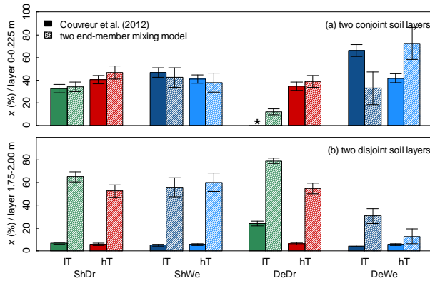
Figure 56: Comparison between relative contributions to transpiration ( x , in %) simulated by the analytical RWU model of Couvreur et al. (2012) and the two end-member mixing model in case of two defined soil layers. Figure 5a displays x from the topmost soil layer (0 – 0.225 m) in case of a two conjoint soil layers (0 – 0.225 m and 0.225 – 2.00 m) whereas Figure 5b displays x from the lowest soil layer (1.75 – 2.00 m) in case of a two disjoint soil layers (0 – 0.225 m and 0.225 – 2.00 m), i.e., information on soil water isotopic composition is lacking between 0.225 and 1.75 m. “Sh” (“De”) stands for the virtual experiments where the soil has a shallow (deep) groundwater table while “Dr” and “We” stand for when the soil is dry or wet at the surface. Suffices “IT” and “hT” refer to “low” and “high” transpiration rate simulations. “*” refers to when hydraulic redistribution is simulated by the analytical model, leading to a negative x . Error bars are either one standard deviation (for the RWU analytical model) or one standard error (for the TM approach).
