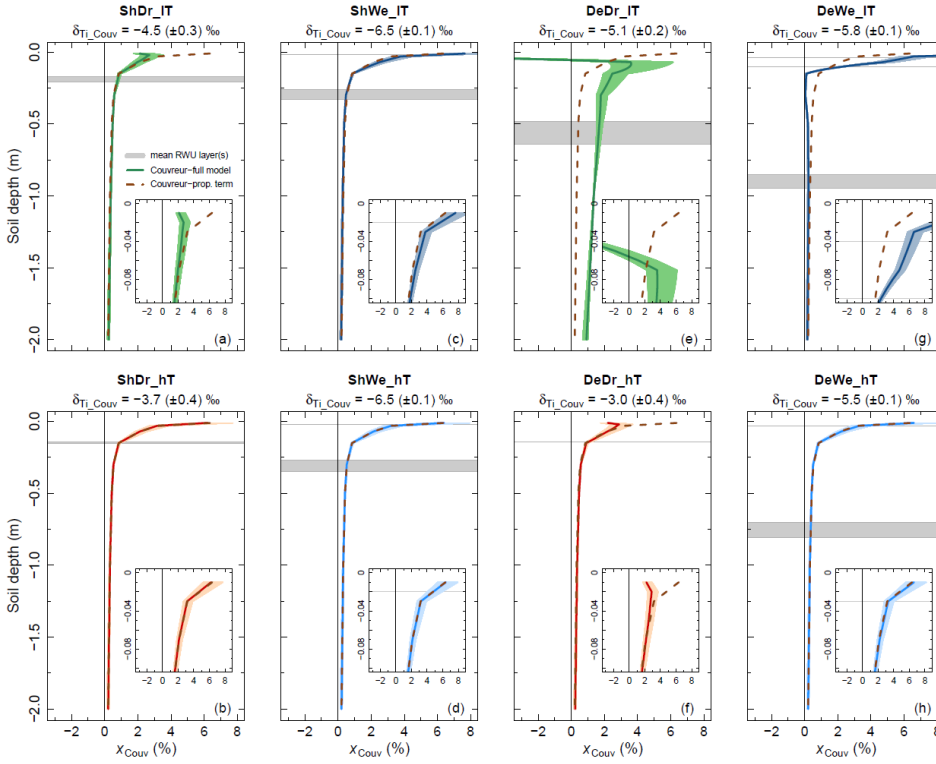
2 3 Figure 45: Simulated depth ( z , in m) profiles of x_{Couv} (%) (solid colored lines), the simulated relative contributions to 4 transpiration provided by the model of Couvreur et al. (2012) for experiments “ShDr” (soil with shallow groundwater 5 table and relatively dry soil surface), “ShWe” (soil with shallow groundwater table after a rainfall event), “DeDr” 6 (soil with deep groundwater table with relatively dry soil surface), “DeWe” (soil with deep groundwater table and wet 7 soil surface). Suffices “IT” and “hT” refer to “low” and “high” transpiration rate simulations. The color-shaded areas 8 depict the uncertainty of the model estimates on the account of the precision of the measurements. The horizontal 9 gray-shaded areas delimit the mean root water uptake layer(s) obtained by the “graphical inference” method. At the 10 bottom right corner of each plot is a detail presented for z \geq -0.10 m. Finally, results from the first term of the model 11 of Couvreur et al. (2012) which considers uptake proportional to root length density is plotted as a dashed brown line 12 for comparison. Note that negative x_{Couv} means hydraulic redistribution by the roots.
