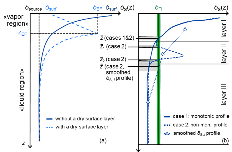
2 3 4 5 6 7 8 9 Figure 2: (a) Simulated soil water isotopic composition ( \delta_s ) profiles for a water-saturated (dark blue line) and unsaturated (light blue dotted line) soil following Barnes and Allison (1983). Indices “surf” and “EF” refer to soil surface and Evaporation Front. “vapor” and “liquid” regions refer to soil regions where water flow occurs predominantly in the liquid and vapor phase, respectively. (b) Illustration of the “graphical inference” method for determining the “mean root water uptake depth” ( \bar{z} ). “Ti” stands for the sap xylem water at the plant tiller. Case 1: one unique solution is found; case 2: more than one solution is found. Smoothed profile is designated by the symbols \triangle . \bar{z} range is indicated by the gray horizontal stripes.
