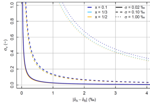
2 3 | Figure 34: Standard error ( \sigma_x ) associated with the estimation of the relative contribution ( x ) of source A water to root 4 water uptake in case of two distinct sources (A and B of isotopic compositions \delta_A and \delta_B ). Three x values (0.1, dark 5 blue color; 1/3, light blue; 1/2, orange) and three values of standard errors associated with sampling and measurement 6 of \delta_A , \delta_B , and of the isotopic composition of the tiller sap water ( \delta_{Ti} ) (0.02, solid line; 0.10 and 1.00, dashed lines) are 7 tested.
