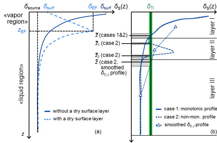
Figure 2: (a) Simulated soil water isotopic composition ( \delta_s ) profiles for a water saturated (dark blue line) and unsaturated (light blue dotted line) soil following Barnes and Allison (1983). Indices “surf” and “EF” refer to soil surface and Evaporation Front. “vapor” and “liquid” regions refer to soil regions where water flow occurs predominantly in the liquid and vapor phase, respectively. (b) Illustration of the “graphical inference” method for determining the “mean root water uptake depth” ( \bar{z} ). “Ti” stands for the sap xylem water at the plant tiller. Case 1: one unique solution is found; case 2: more than one solution is found. Smoothed profile is designated by the symbols). \bar{z} range is indicated by the gray horizontal stripes.
