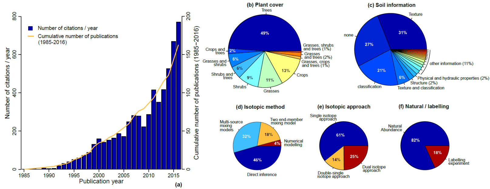
2 3 Figure 3: Results of the literature review when entering the search terms ("root water uptake" or ("water source" and root) or "water uptake") and isotop*) into the ISI Web of 4 Science search engine (www.webofknowledge.com): (a) Evolution of the number of citations per year and cumulative number of publications from 1985 to 2016; (b) details are given 5 on the plant cover; (c) the available soil information; (d) the applied isotopic method and (e) approach, and the type of experiment (f).
