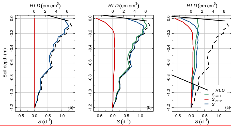
5 Figure 1: Some examples of root water uptake sink term ( S , in d^{-1} ) profiles (blue lines) conceptualized as the sum of 6 S_{uniH} (green lines), the root water uptake term proportional to root length density RLD (dotted black line) and the 7 compensatory root water uptake ( S_{comp} , red lines). (a) S_{comp} = 0 (no root compensation) leading to S = S_{uniH} . (b) S_{comp} \neq 8 0 and becomes negative towards the surface but remains smaller (in absolute term) than S_{uniH} . (c) S_{comp} \neq 0 and is 9 negative at the surface while is greater than S_{uniH} for z > -0.08 m. In the last case, S is negative at the surface, meaning 10 hydraulic lift is observed.
