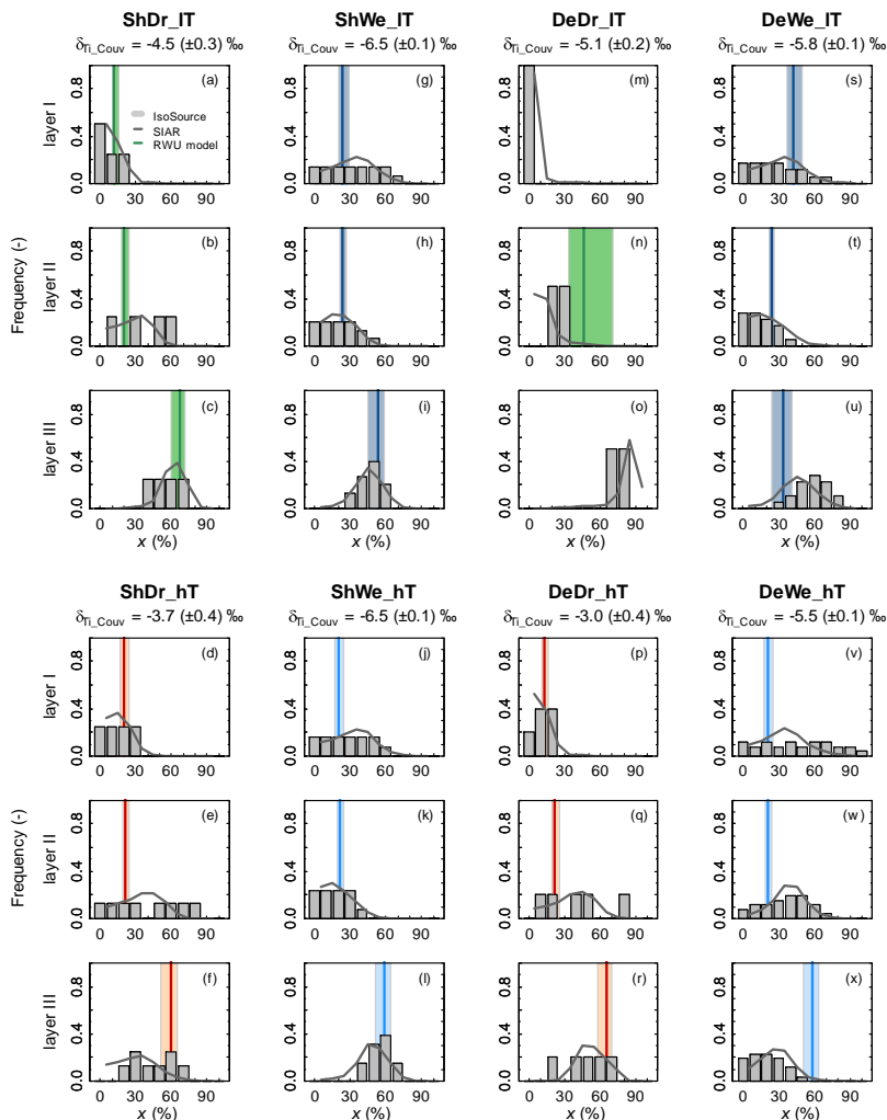
Figure 67: Simulated ranges of possible relative contributions to transpiration from three defined soil layers (I: 0.00 – 0.05 m, II: 0.050 – 0.225 m, and III: 0.225 – 2.000) provided by the multi-source mixing model IsoSource (Phillips and Gregg, 2003) (displayed in the form of gray histograms). Density distribution functions following the Bayesian model SIAR (Parnell et al., 2010) (gray lines). “Sh” (“De”) stands for the virtual experiments where the soil has a shallow (deep) groundwater table while “Dr” and “We” stand for when the soil is dry or wet at the surface. Suffices “IT” and “hT” refer to “low” and “high” transpiration rate simulations. The colored vertical lines give x_{I\_Couv} , x_{II\_Couv} , and x_{III\_Couv} , the relative contributions to transpiration from layers I, II, and III simulated by the analytical model of Couvreur et al. (2012). The color-shaded areas associated with x_{I\_Couv} , x_{II\_Couv} , and x_{III\_Couv} refer to their uncertainty associated with input data uncertainty.
