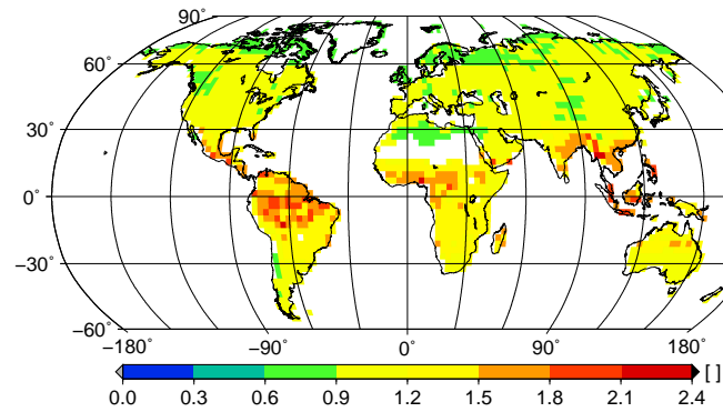
Figure 4. Global patterns of the ratio of respiration to NPP. Ratio of respiration to NPP of lichens and bryophytes estimated by LiBry for a) all locations of growth, b) the canopy and c) the ground.
