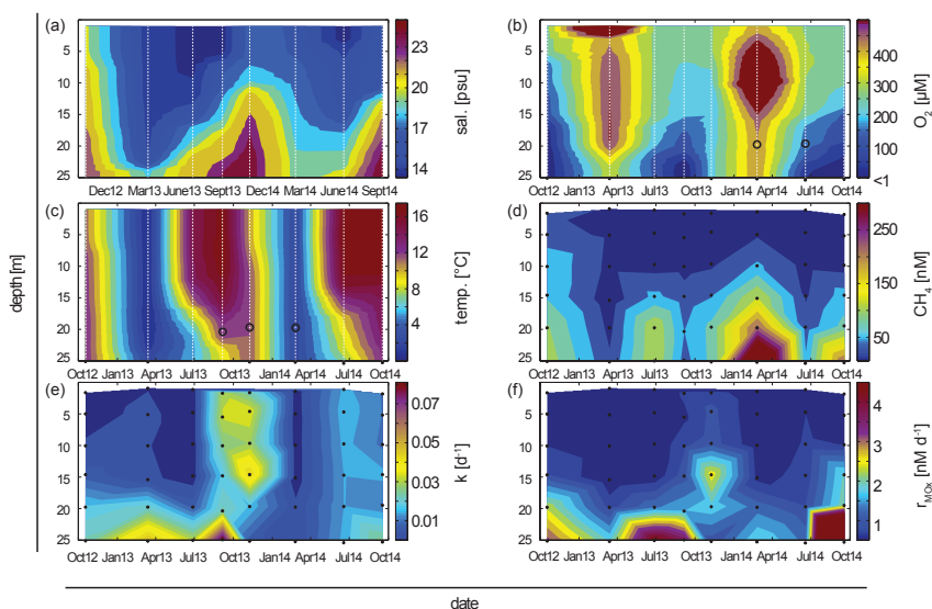
10 Figure 2. Seasonal variability of physico-chemical parameters and aerobic methanotrophy at the Boknis Eck station. Distribution of salinity (a), oxygen (b), temperature (c), methane (d), first order rate constants of aerobic methane oxidation k (e), and aerobic methane oxidation rates r_{MOx} (f). Positions of discrete samples (dots) and continuous measurements (dashed lines) are indicated. Depths of water used for oxygen and temperature incubation experiments (Fig. 3, 4 and 5) are indicated with circles in (b) and (c).
