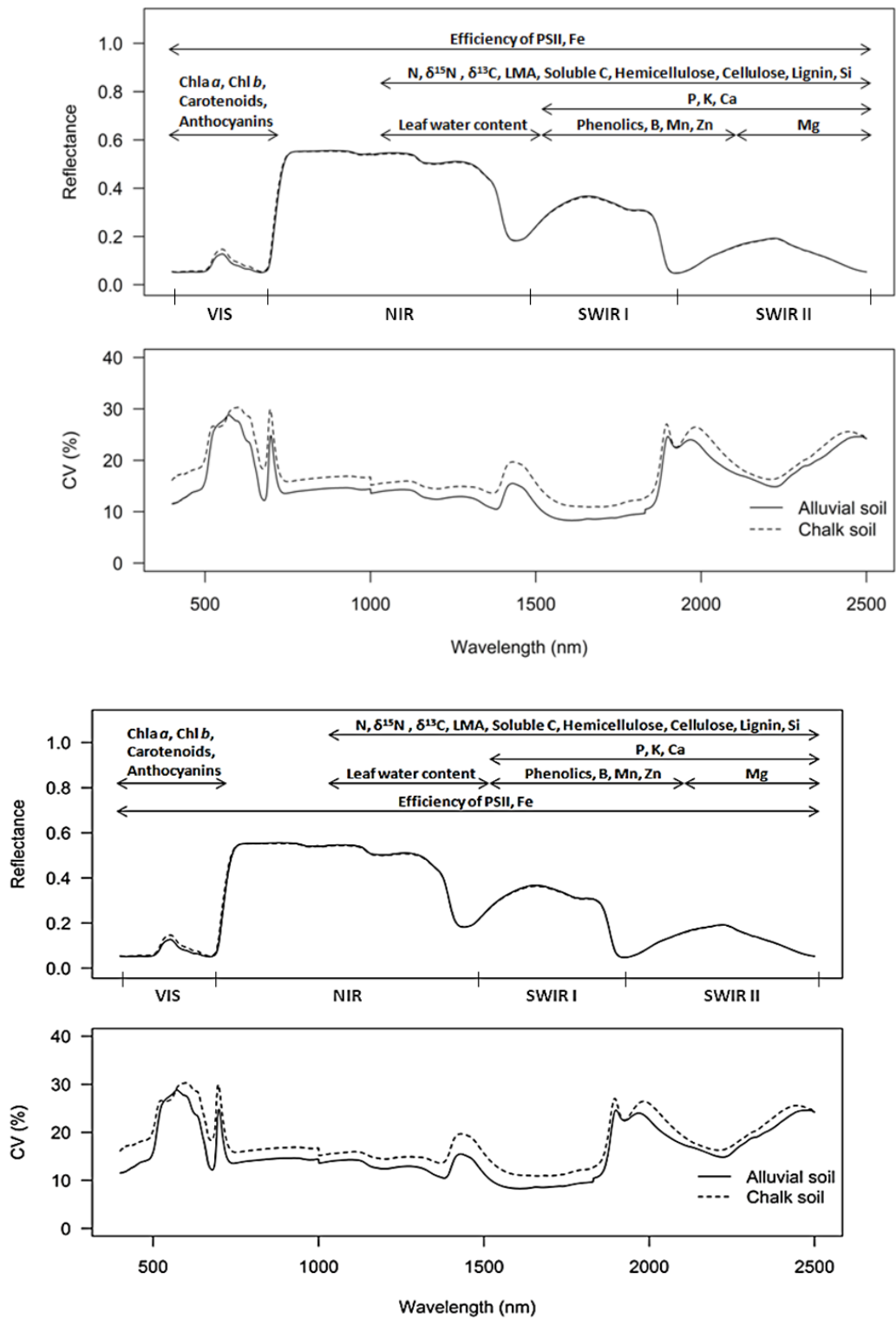
Figure 3. Spectral reflectance and percentage coefficient of variation (CV) of reflectance of six generalists species for alluvial and chalk soils. The spectral regions for each trait were selected based on the model that minimised RMSE.
