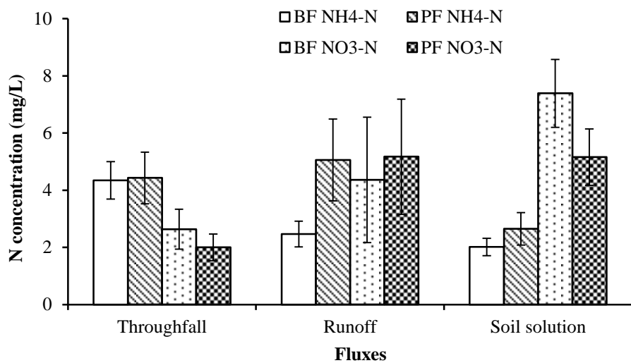
Fig. 1 Mean concentration (mg N/L) of \text{NH}_4^+ -N and \text{NO}_3^- -N in throughfall, surface runoff and seepage below 20 cm sampled from September 2012 to February 2013. Error bars indicate SE of plot means ( n = 3 ).
