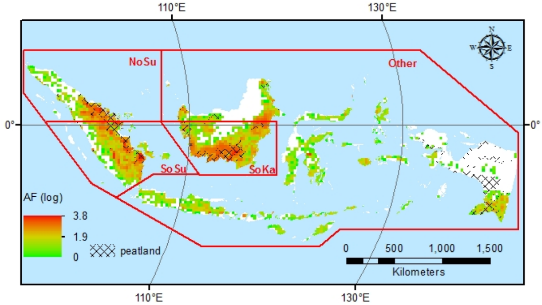
Figure 1: Region definition, number of active fires detected between 1997 and 2015 (log scale, rescaled to quarter degree) and peatland extent for Indonesia. NoSu is northern Sumatra, SoSu southern Sumatra, and SoKa is southern Kalimantan. The white areas are where no active fires were detected.
