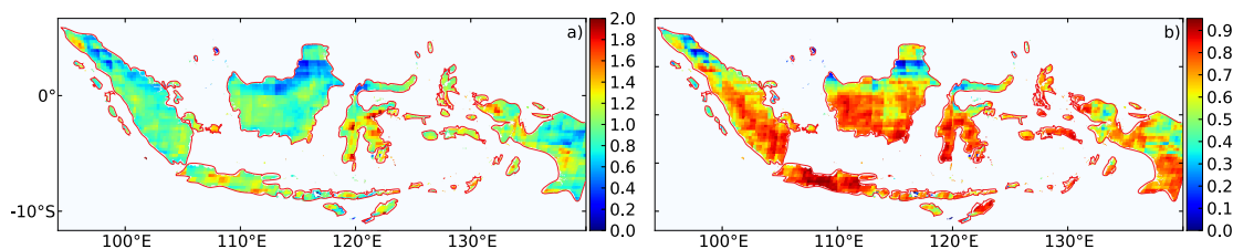
635 Figure 2: a) Slope and b) R^2 of a linear regression between GPCP and TRMM rainfall based on the cumulated rainfall for the 4 driest months between 1998 and 2014.
