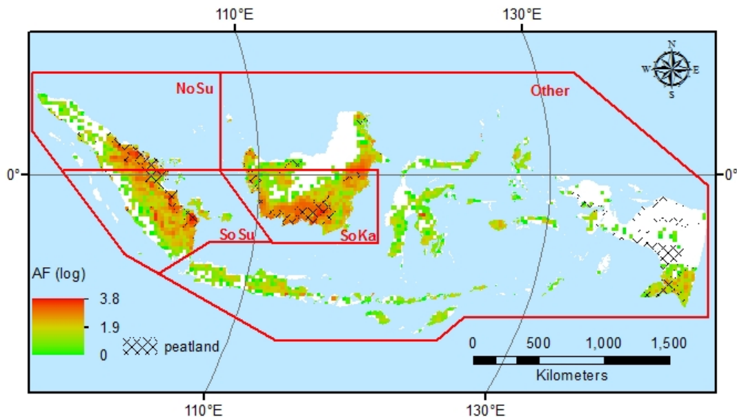
630 Figure 1: Region definition, number of active fires detected between 1997 and 2015 (log scale, rescaled to quarter degree) and peatland extent for Indonesia. NoSu is northern Sumatra, SoSu southern Sumatra, and SoKa is southern Kalimantan. The white areas are where no active fires were detected.
