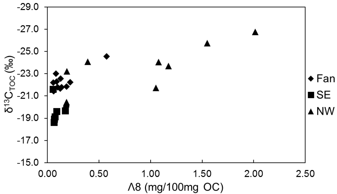
Figure 6: Stable carbon isotopic composition of total organic carbon ( \delta^{13}\text{C}_{\text{TOC}} ) vs. carbon-normalized lignin content ( \Lambda 8 ) for marine surface sediment samples from the Amazon continental margin.
