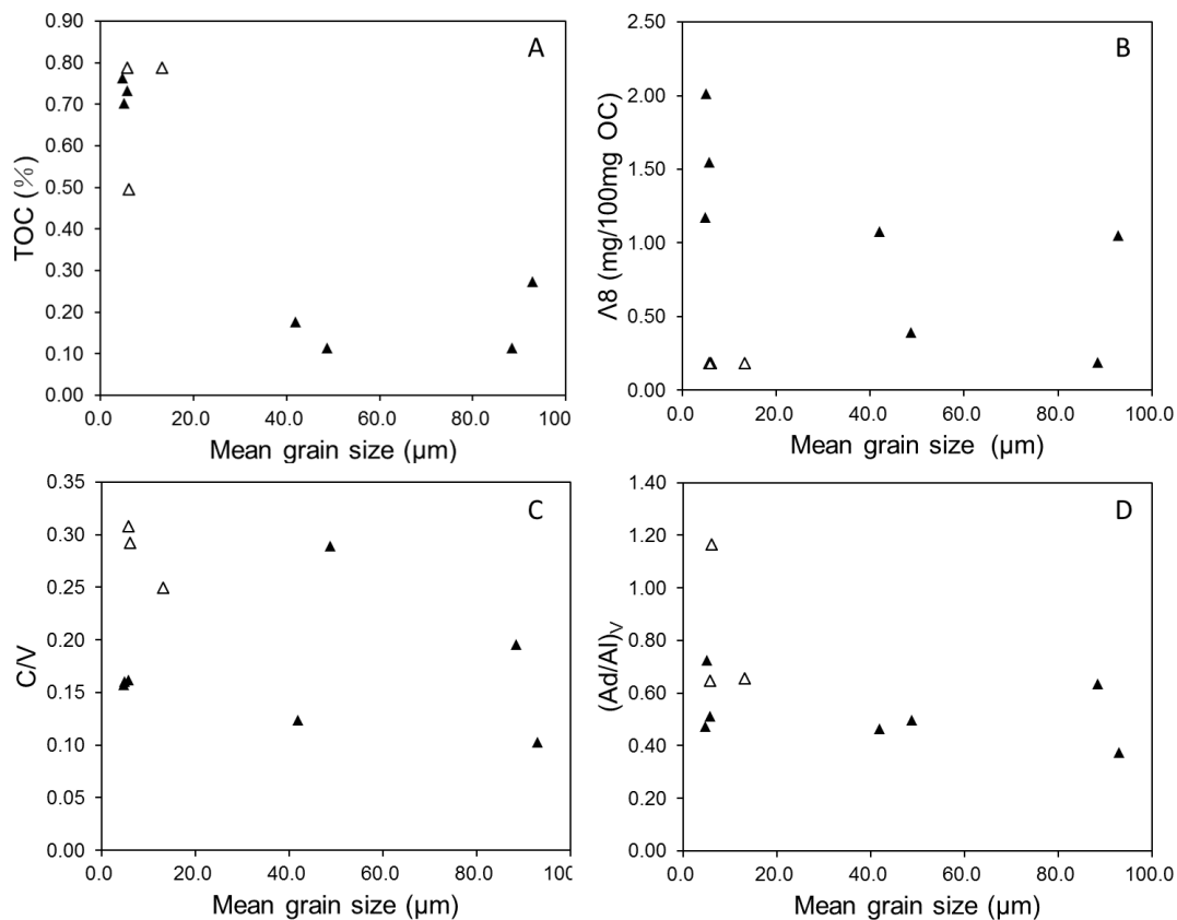
Figure 7: A), B), C) and D) indicate total organic carbon (TOC) content, carbon-normalized lignin content ( \Lambda 8 ), cinnamyl:vanillyl (C/V) ratio and lignin degradation index ( (Ad/Al)_v ) for marine surface sediment samples from the NW sector vs. mean grain size, respectively. Empty triangles represent the three deepest sites (>2000 m) far from the coast, and filled triangles represent the other sites in the NW sector with water depth shallower than 100 m. See Table 2 and Fig. 5 for the location of the NW sector.
