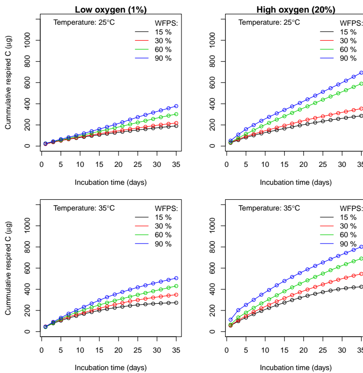
Fig. 1. Cumulative respiration for all treatments in the incubation experiment.
